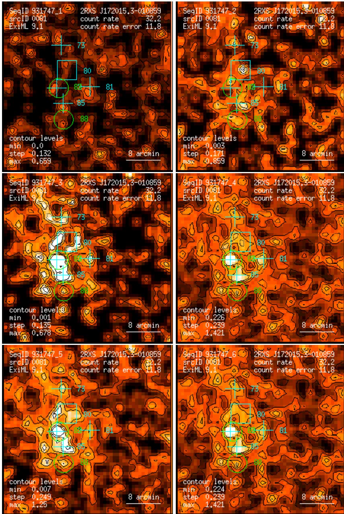
Figure 81: RASS 931747: detection 0081: band rate images, Gaussian filter: (1) PSPC channels 11 – 41, (2) 52 – 90, (3) 91 – 201, (4) 11 – 235, (5) 52 – 201, (6) 11 – 201. Broad band rates in counts/ks. Band rate contour levels in counts/ks/arcmin 2 .
