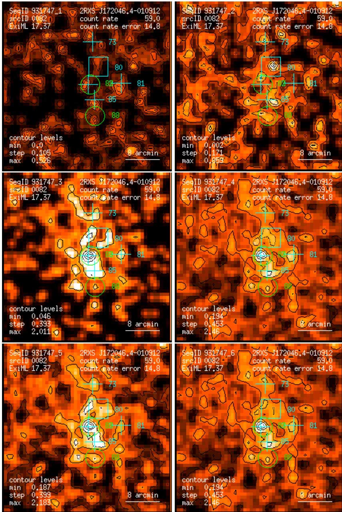
Figure 82: RASS 931747: detection 0082: band rate images, Gaussian filter: (1) PSPC channels 11 – 41, (2) 52 – 90, (3) 91 – 201, (4) 11 – 235, (5) 52 – 201, (6) 11 – 201. Broad band rates in counts/ks. Band rate contour levels in counts/ks/arcmin 2 .
