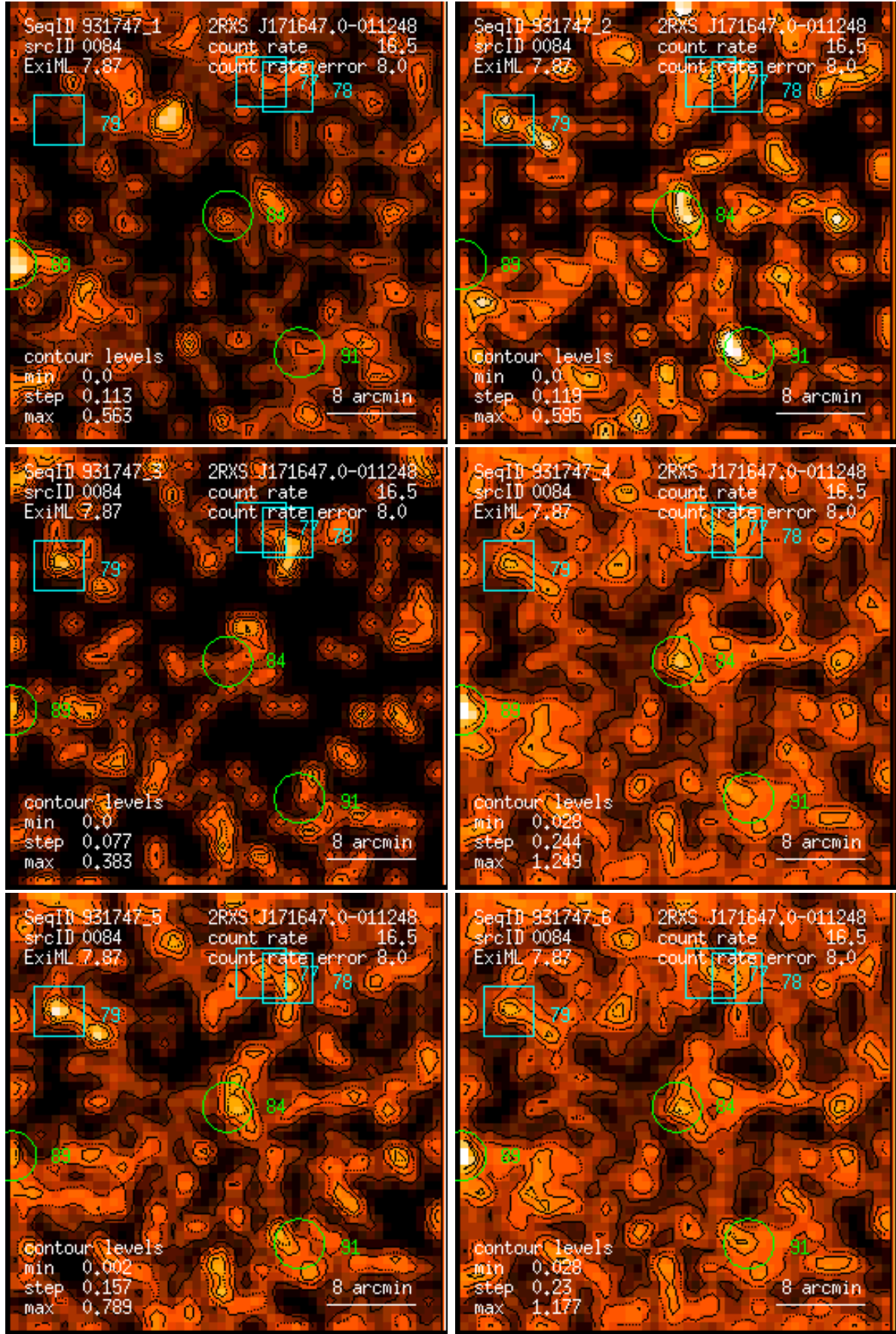
Figure 84: RASS 931747: detection 0084: band rate images, Gaussian filter: (1) PSPC channels 11 – 41, (2) 52 – 90, (3) 91 – 201, (4) 11 – 235, (5) 52 – 201, (6) 11 – 201. Broad band rates in counts/ks. Band rate contour levels in counts/ks/arcmin 2 .
