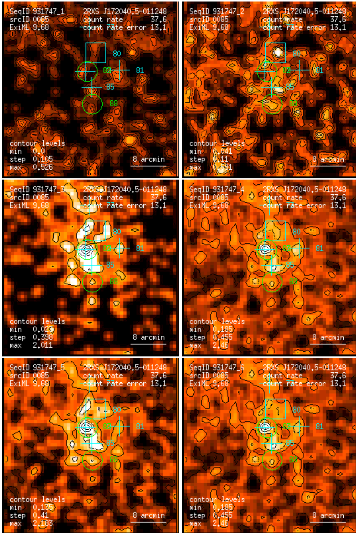
Figure 85: RASS 931747: detection 0085: band rate images, Gaussian filter: (1) PSPC channels 11 – 41, (2) 52 – 90, (3) 91 – 201, (4) 11 – 235, (5) 52 – 201, (6) 11 – 201. Broad band rates in counts/ks. Band rate contour levels in counts/ks/arcmin 2 .
