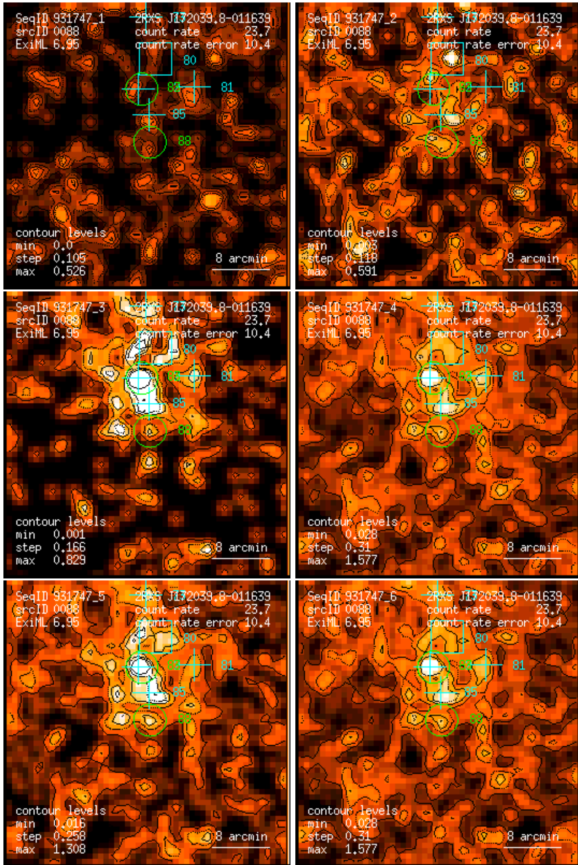
Figure 88: RASS 931747: detection 0088: band rate images, Gaussian filter: (1) PSPC channels 11 – 41, (2) 52 – 90, (3) 91 – 201, (4) 11 – 235, (5) 52 – 201, (6) 11 – 201. Broad band rates in counts/ks. Band rate contour levels in counts/ks/arcmin 2 .
