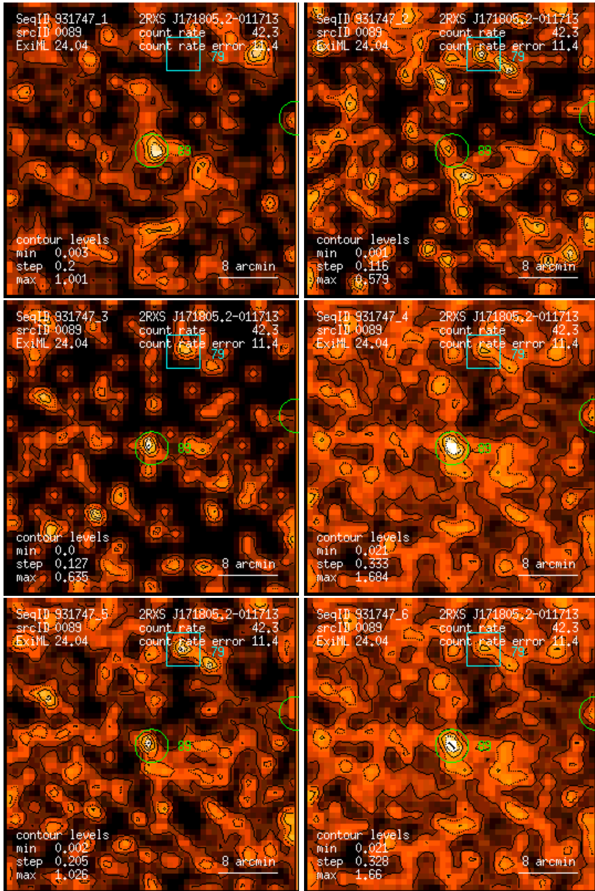
Figure 89: RASS 931747: detection 0089: band rate images, Gaussian filter: (1) PSPC channels 11 – 41, (2) 52 – 90, (3) 91 – 201, (4) 11 – 235, (5) 52 – 201, (6) 11 – 201. Broad band rates in counts/ks. Band rate contour levels in counts/ks/arcmin 2 .
