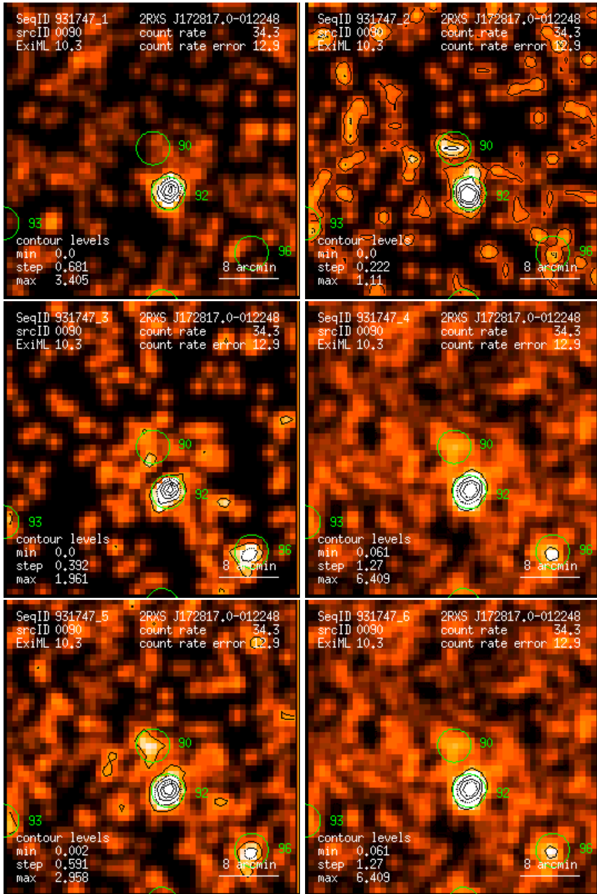
Figure 90: RASS 931747: detection 0090: band rate images, Gaussian filter: (1) PSPC channels 11 – 41, (2) 52 – 90, (3) 91 – 201, (4) 11 – 235, (5) 52 – 201, (6) 11 – 201. Broad band rates in counts/ks. Band rate contour levels in counts/ks/arcmin 2 .
