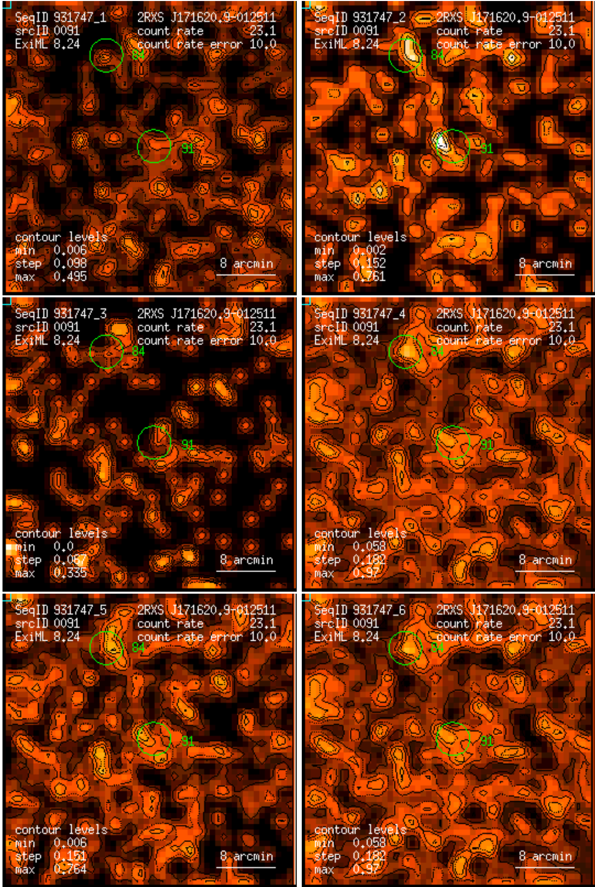
Figure 91: RASS 931747: detection 0091: band rate images, Gaussian filter: (1) PSPC channels 11 – 41, (2) 52 – 90, (3) 91 – 201, (4) 11 – 235, (5) 52 – 201, (6) 11 – 201. Broad band rates in counts/ks. Band rate contour levels in counts/ks/arcmin 2 .
