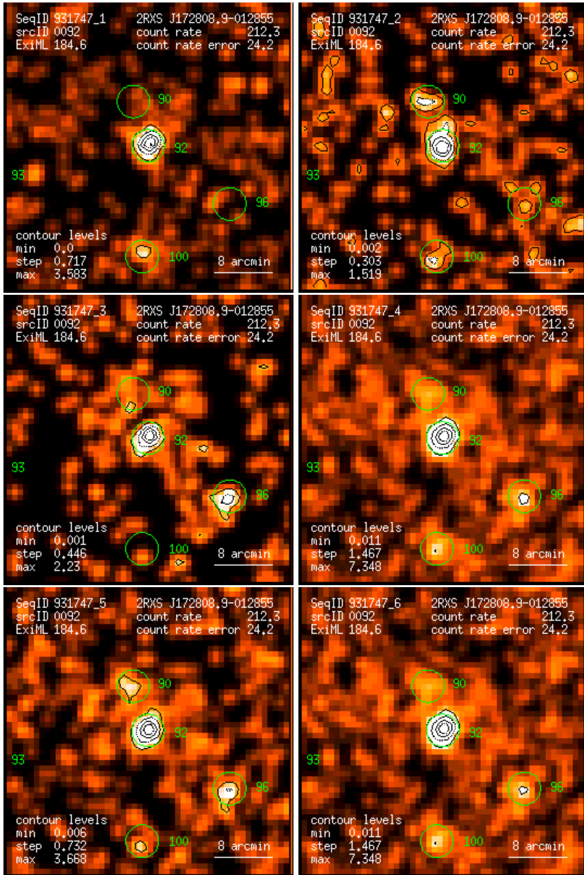
Figure 92: RASS 931747: detection 0092: band rate images, Gaussian filter: (1) PSPC channels 11 – 41, (2) 52 – 90, (3) 91 – 201, (4) 11 – 235, (5) 52 – 201, (6) 11 – 201. Broad band rates in counts/ks. Band rate contour levels in counts/ks/arcmin 2 .
