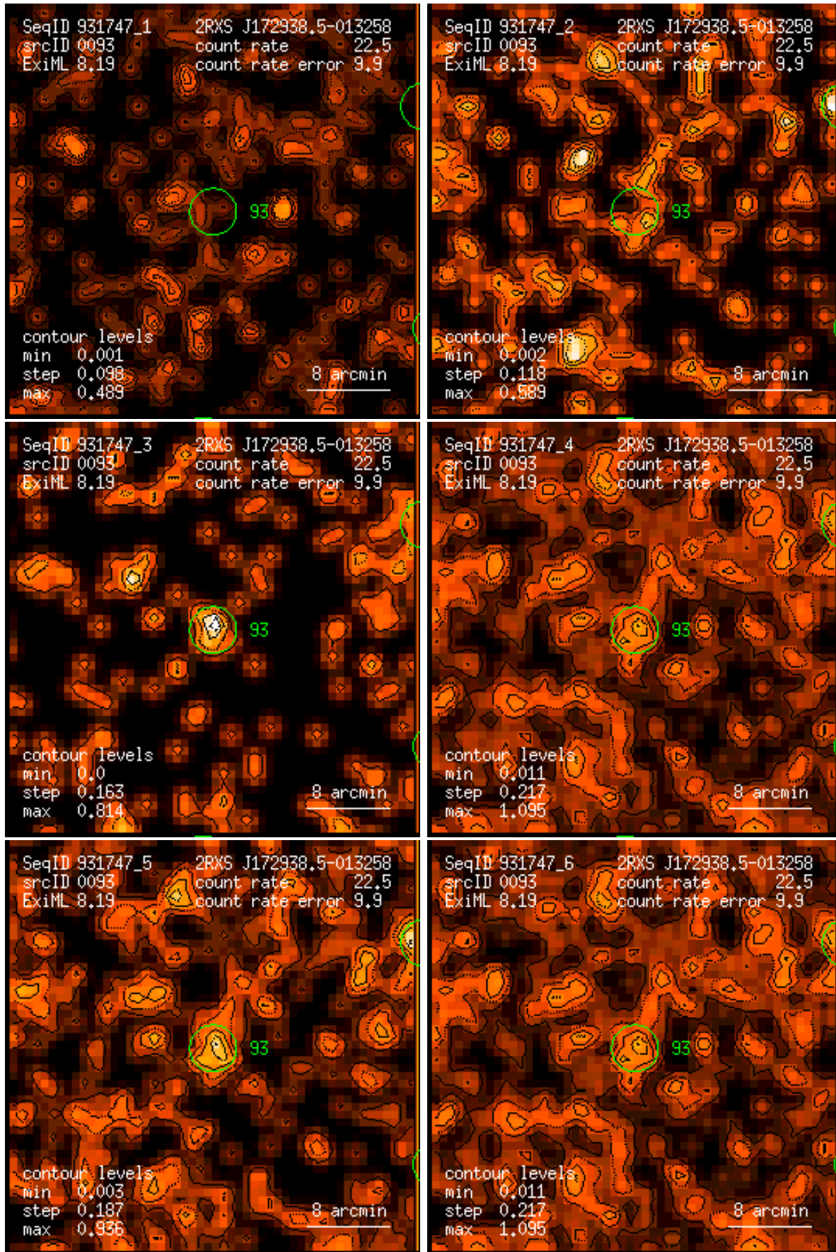
Figure 93: RASS 931747: detection 0093: band rate images, Gaussian filter: (1) PSPC channels 11 – 41, (2) 52 – 90, (3) 91 – 201, (4) 11 – 235, (5) 52 – 201, (6) 11 – 201. Broad band rates in counts/ks. Band rate contour levels in counts/ks/arcmin 2 .
