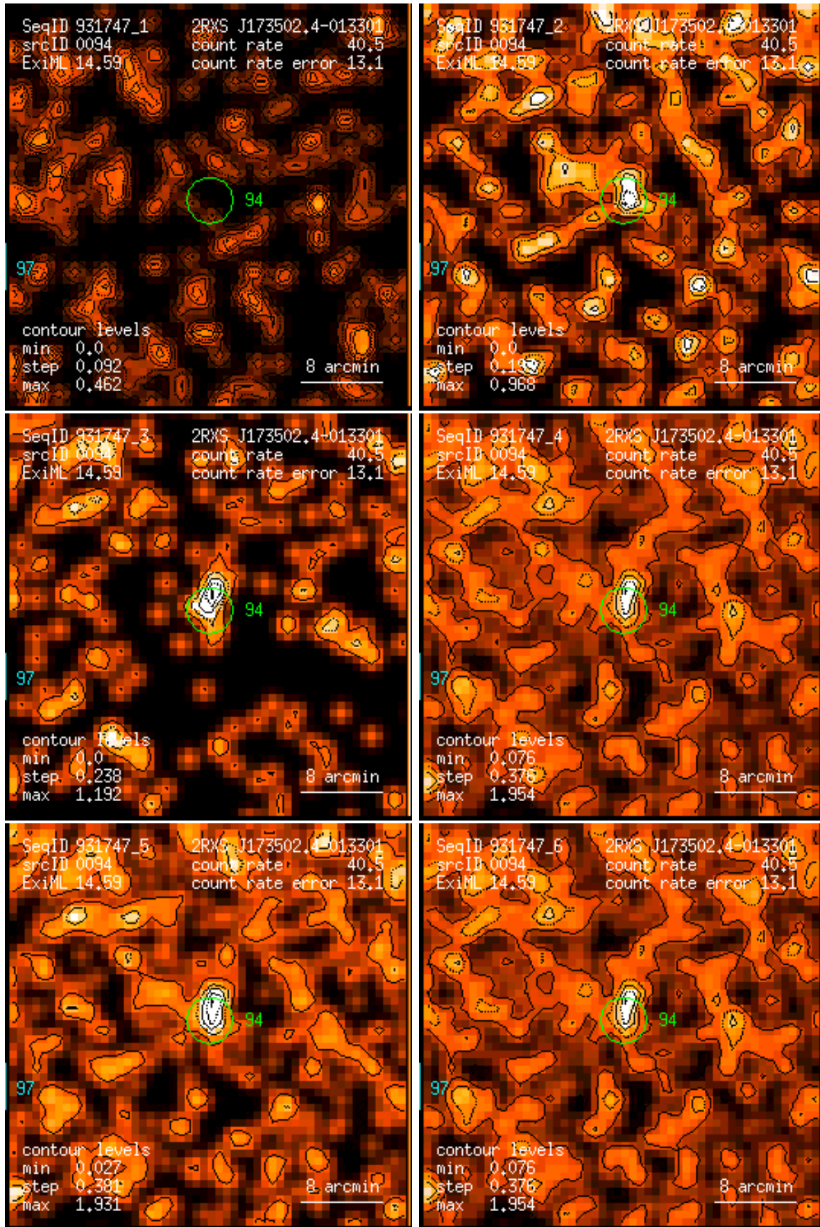
Figure 94: RASS 931747: detection 0094: band rate images, Gaussian filter: (1) PSPC channels 11 – 41, (2) 52 – 90, (3) 91 – 201, (4) 11 – 235, (5) 52 – 201, (6) 11 – 201. Broad band rates in counts/ks. Band rate contour levels in counts/ks/arcmin 2 .
