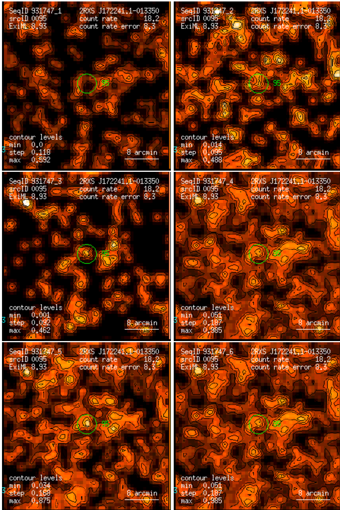
Figure 95: RASS 931747: detection 0095: band rate images, Gaussian filter: (1) PSPC channels 11 – 41, (2) 52 – 90, (3) 91 – 201, (4) 11 – 235, (5) 52 – 201, (6) 11 – 201. Broad band rates in counts/ks. Band rate contour levels in counts/ks/arcmin 2 .
