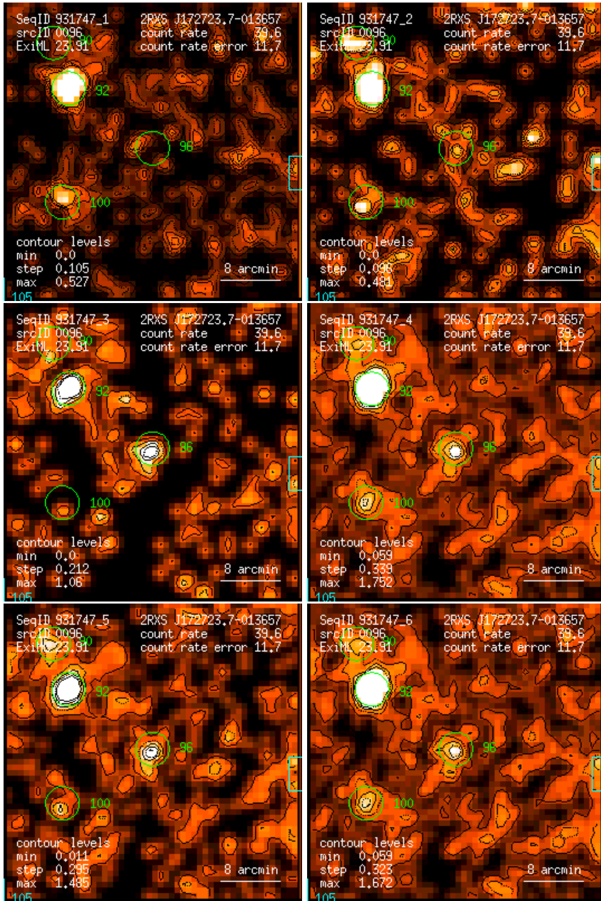
Figure 96: RASS 931747: detection 0096: band rate images, Gaussian filter: (1) PSPC channels 11 – 41, (2) 52 – 90, (3) 91 – 201, (4) 11 – 235, (5) 52 – 201, (6) 11 – 201. Broad band rates in counts/ks. Band rate contour levels in counts/ks/arcmin 2 .
