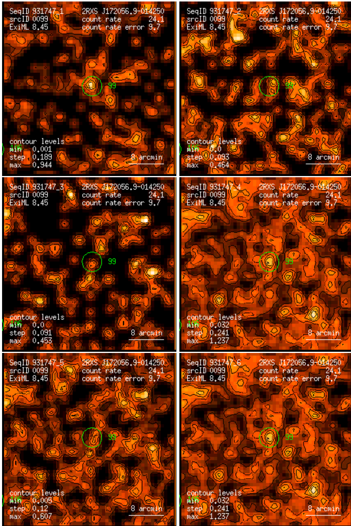
Figure 99: RASS 931747: detection 0099: band rate images, Gaussian filter: (1) PSPC channels 11 – 41, (2) 52 – 90, (3) 91 – 201, (4) 11 – 235, (5) 52 – 201, (6) 11 – 201. Broad band rates in counts/ks. Band rate contour levels in counts/ks/arcmin 2 .
