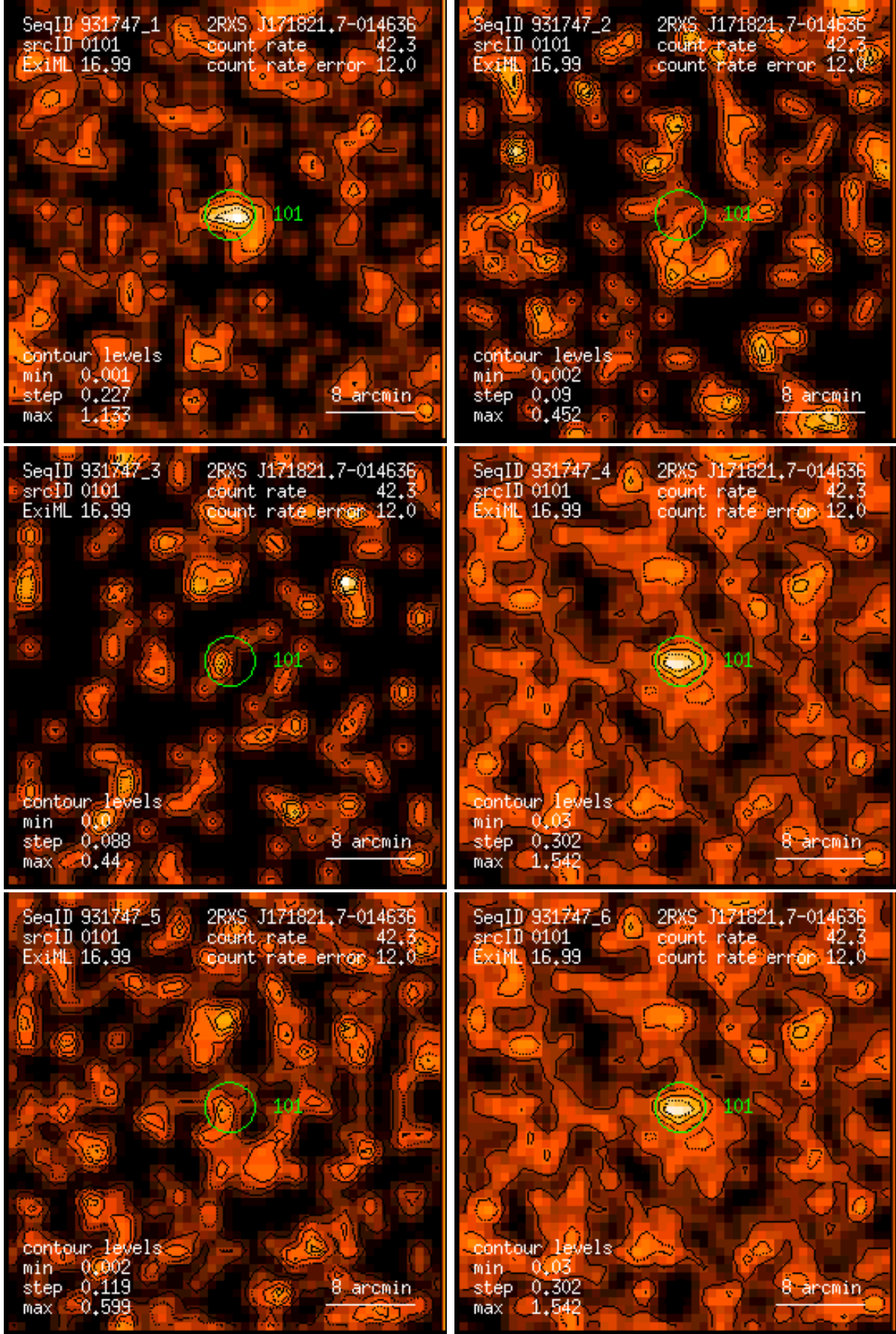
Figure 101: RASS 931747: detection 0101: band rate images, Gaussian filter: (1) PSPC channels 11 – 41, (2) 52 – 90, (3) 91 – 201, (4) 11 – 235, (5) 52 – 201, (6) 11 – 201. Broad band rates in counts/ks. Band rate contour levels in counts/ks/arcmin 2 .
