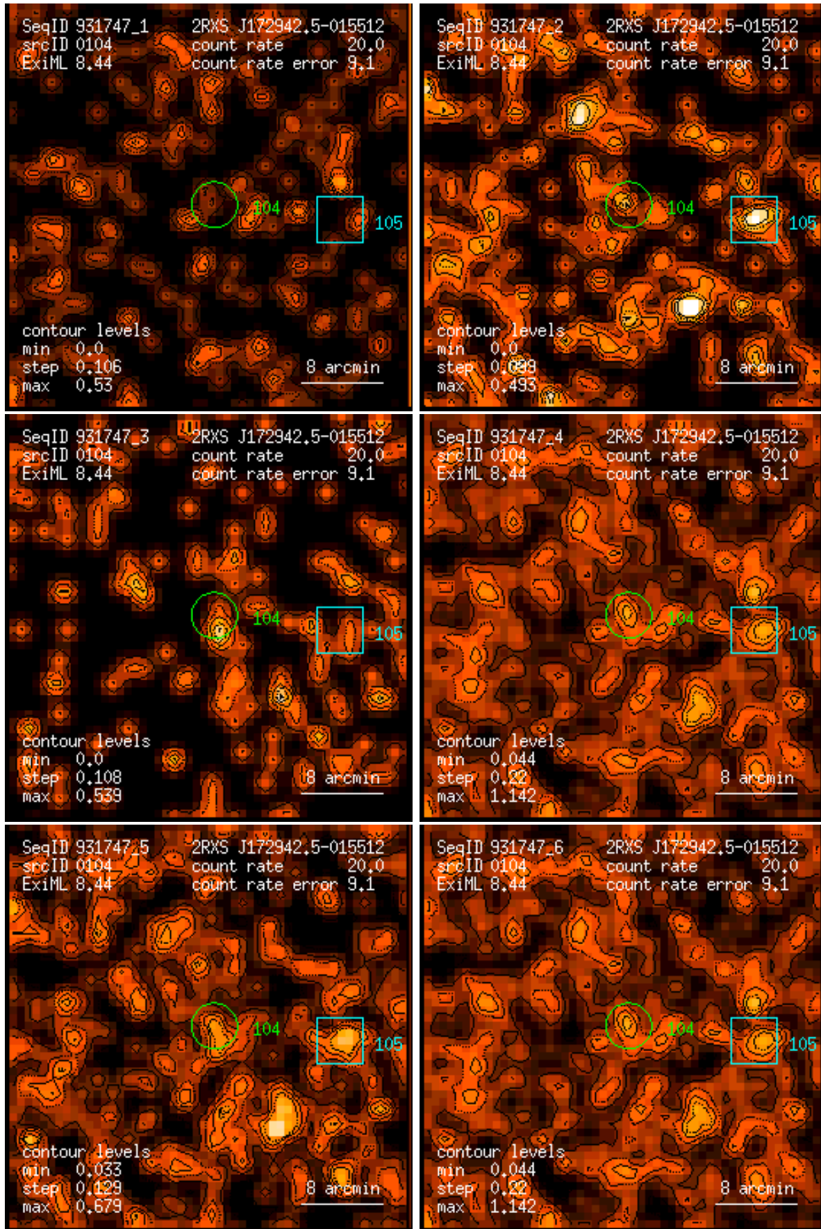
Figure 104: RASS 931747: detection 0104: band rate images, Gaussian filter: (1) PSPC channels 11 – 41, (2) 52 – 90, (3) 91 – 201, (4) 11 – 235, (5) 52 – 201, (6) 11 – 201. Broad band rates in counts/ks. Band rate contour levels in counts/ks/arcmin 2 .
