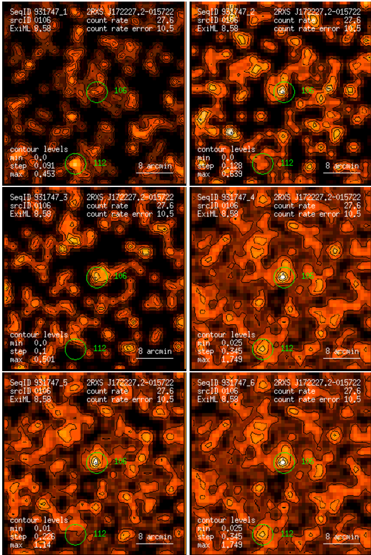
Figure 106: RASS 931747: detection 0106: band rate images, Gaussian filter: (1) PSPC channels 11 – 41, (2) 52 – 90, (3) 91 – 201, (4) 11 – 235, (5) 52 – 201, (6) 11 – 201. Broad band rates in counts/ks. Band rate contour levels in counts/ks/arcmin 2 .
