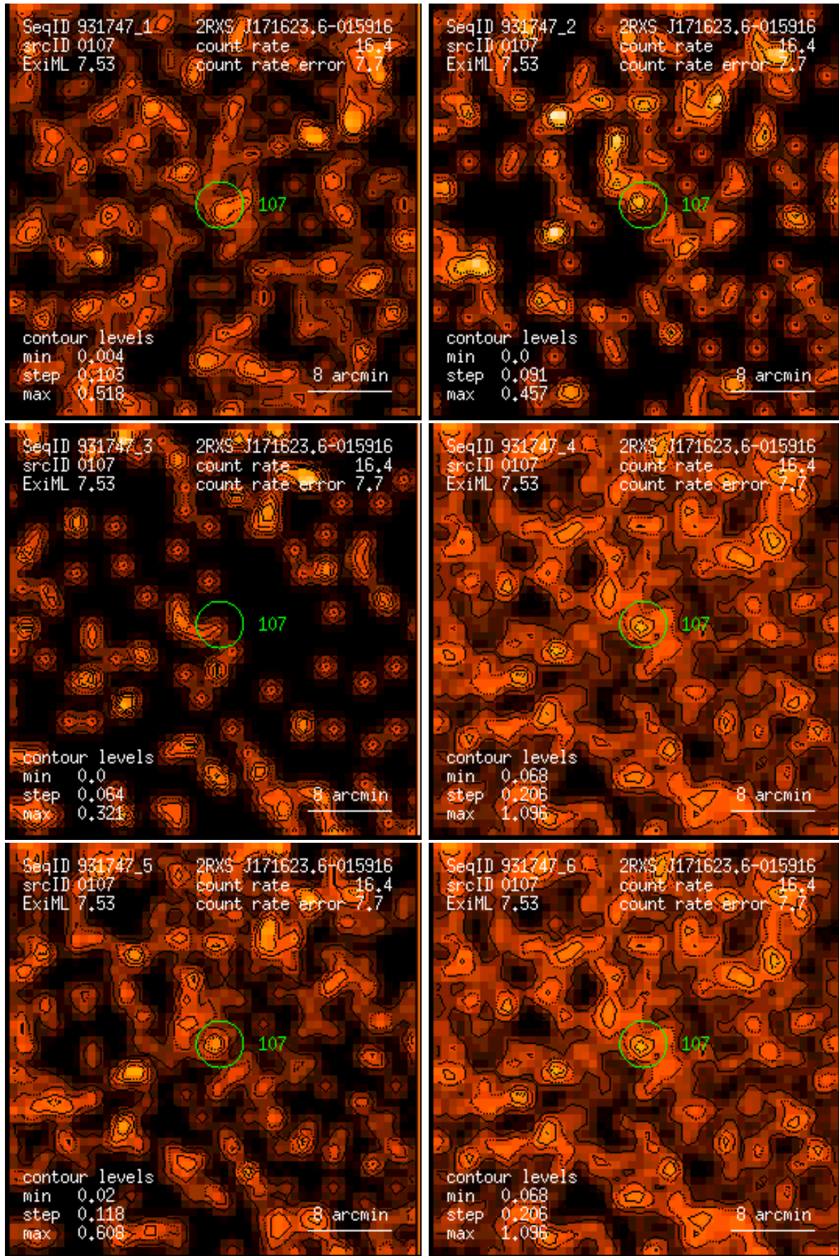
Figure 107: RASS 931747: detection 0107: band rate images, Gaussian filter: (1) PSPC channels 11 – 41, (2) 52 – 90, (3) 91 – 201, (4) 11 – 235, (5) 52 – 201, (6) 11 – 201. Broad band rates in counts/ks. Band rate contour levels in counts/ks/arcmin 2 .
