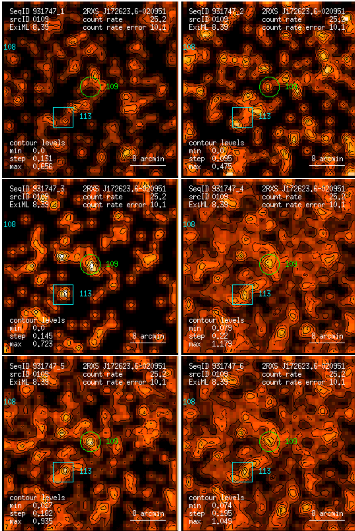
Figure 109: RASS 931747: detection 0109: band rate images, Gaussian filter: (1) PSPC channels 11 – 41, (2) 52 – 90, (3) 91 – 201, (4) 11 – 235, (5) 52 – 201, (6) 11 – 201. Broad band rates in counts/ks. Band rate contour levels in counts/ks/arcmin 2 .
