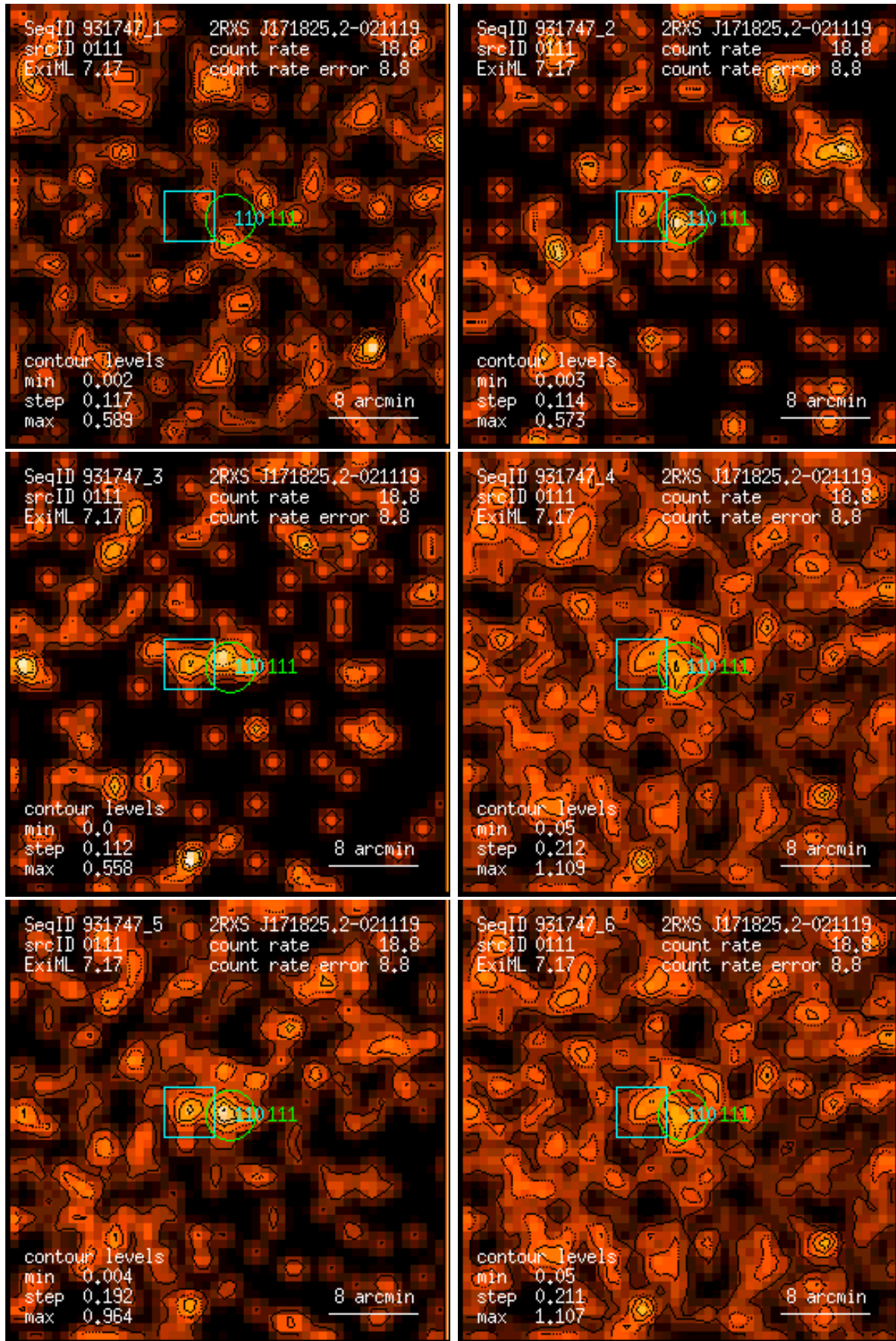
Figure 111: RASS 931747: detection 0111: band rate images, Gaussian filter: (1) PSPC channels 11 – 41, (2) 52 – 90, (3) 91 – 201, (4) 11 – 235, (5) 52 – 201, (6) 11 – 201. Broad band rates in counts/ks. Band rate contour levels in counts/ks/arcmin 2 .
