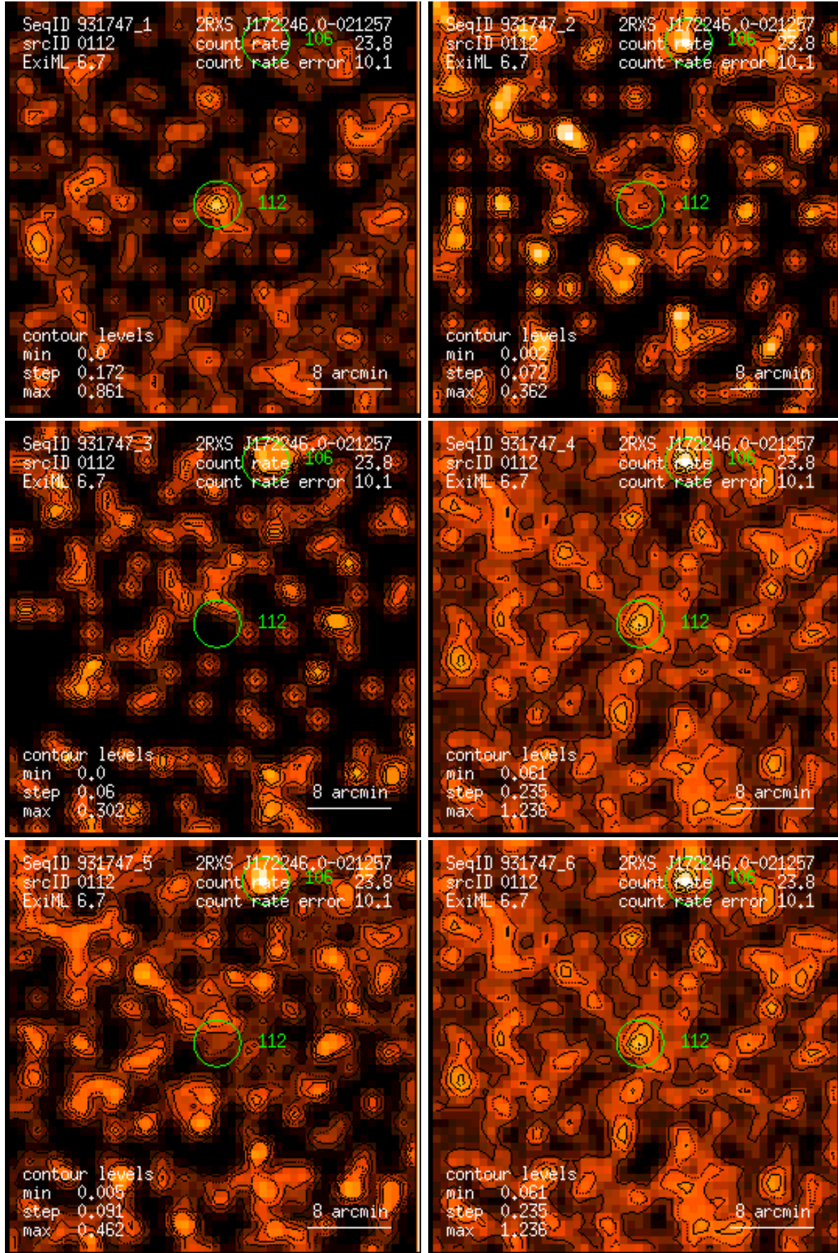
Figure 112: RASS 931747: detection 0112: band rate images, Gaussian filter: (1) PSPC channels 11 – 41, (2) 52 – 90, (3) 91 – 201, (4) 11 – 235, (5) 52 – 201, (6) 11 – 201. Broad band rates in counts/ks. Band rate contour levels in counts/ks/arcmin 2 .
