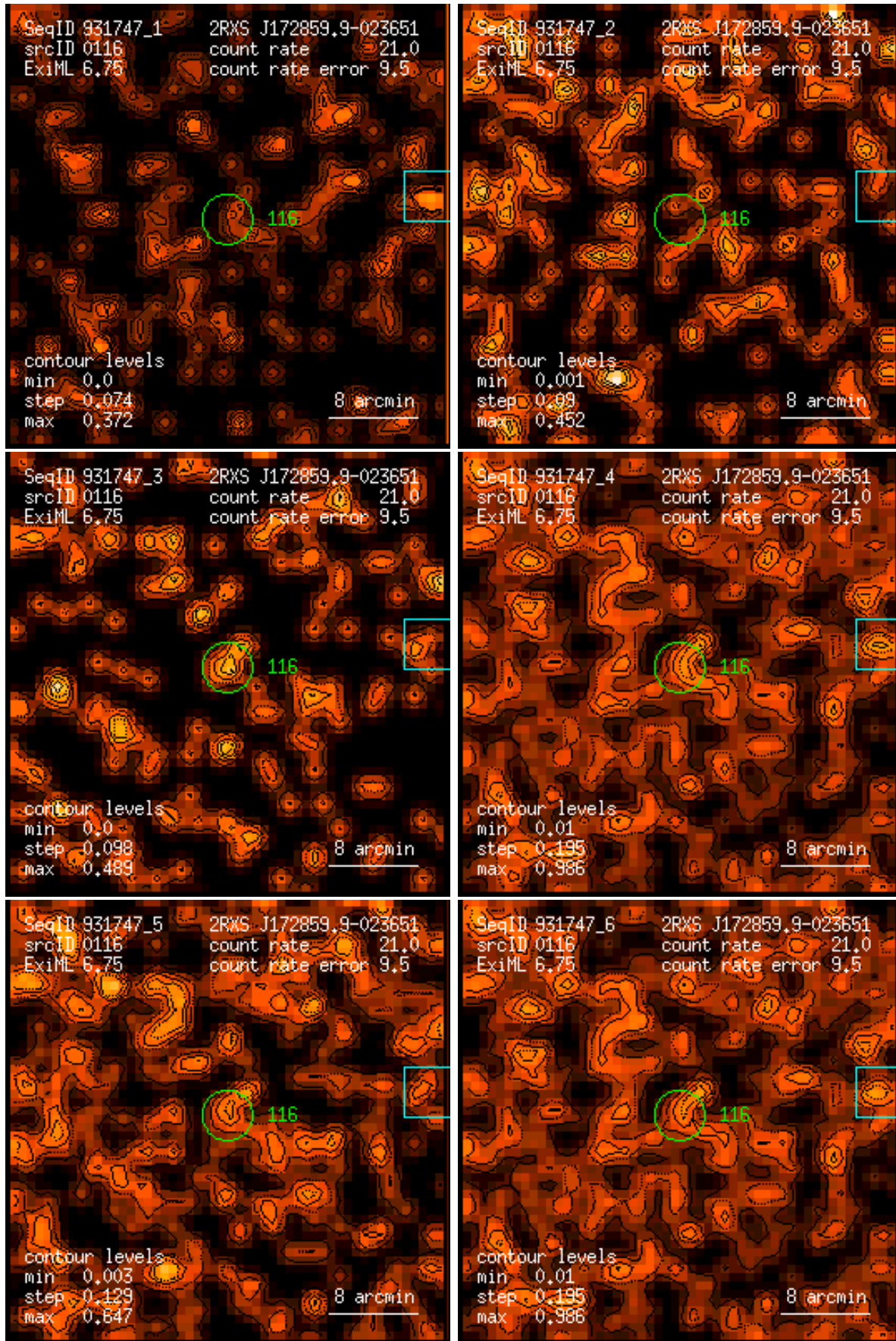
Figure 116: RASS 931747: detection 0116: band rate images, Gaussian filter: (1) PSPC channels 11 – 41, (2) 52 – 90, (3) 91 – 201, (4) 11 – 235, (5) 52 – 201, (6) 11 – 201. Broad band rates in counts/ks. Band rate contour levels in counts/ks/arcmin 2 .
