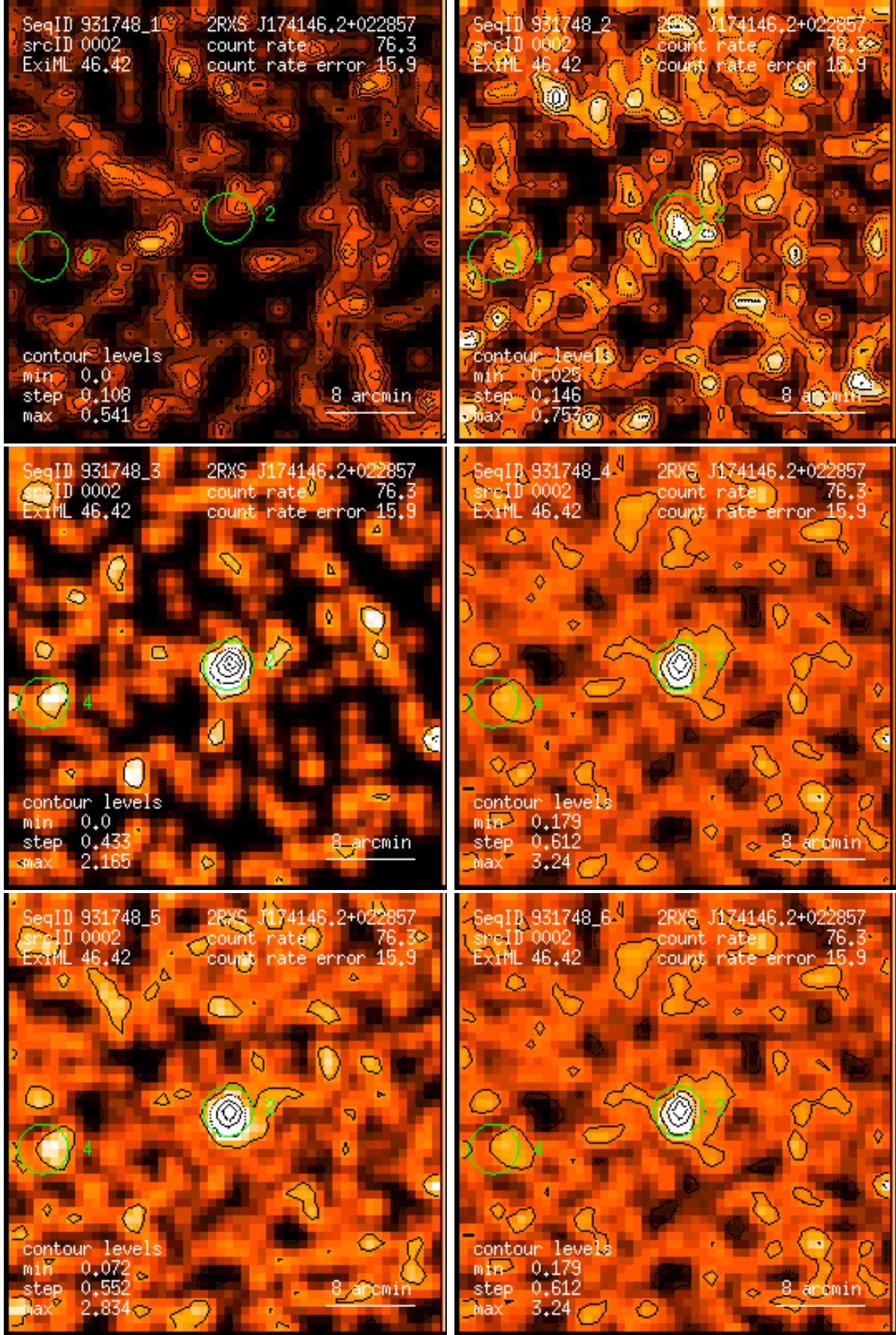
Figure 2: RASS 931748: detection 0002: band rate images, Gaussian filter: (1) PSPC channels 11 – 41, (2) 52 – 90, (3) 91 – 201, (4) 11 – 235, (5) 52 – 201, (6) 11 – 201. Broad band rates in counts/ks. Band rate contour levels in counts/ks/arcmin 2 .
