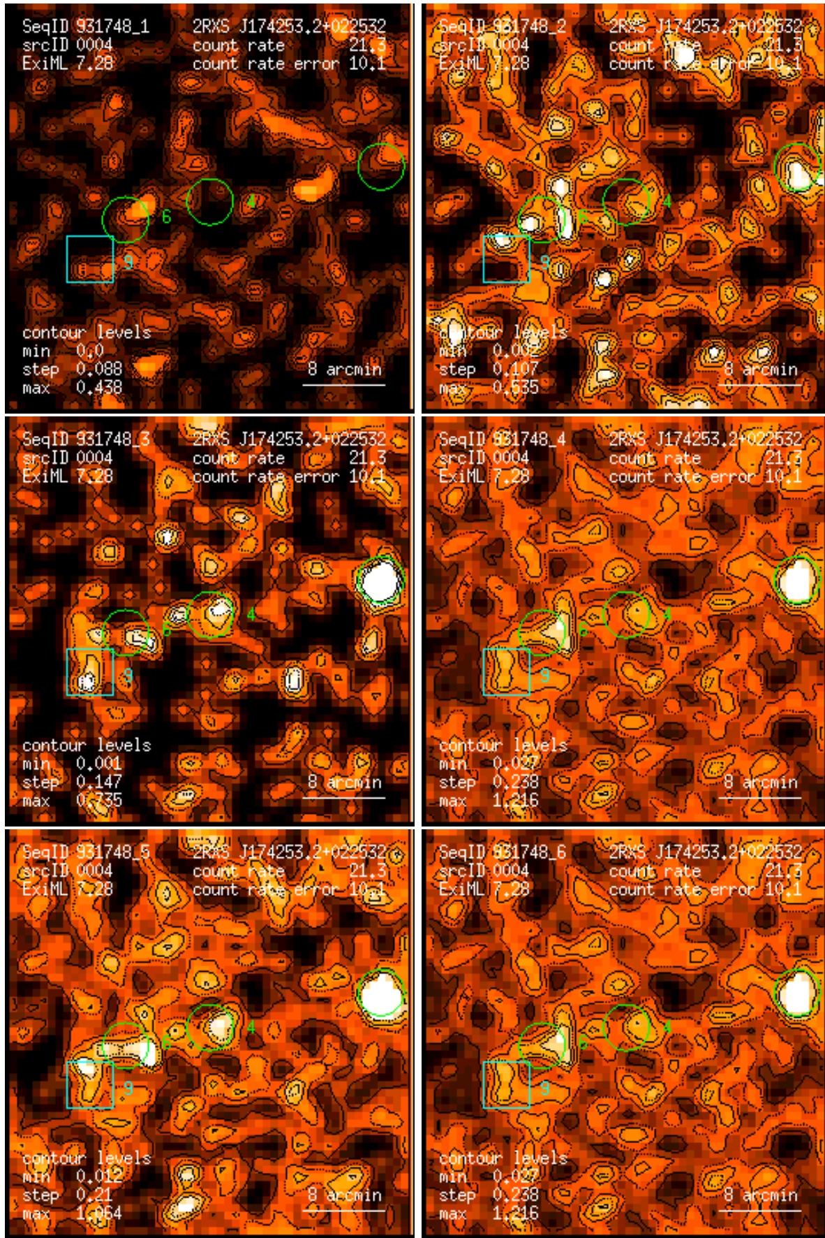
Figure 4: RASS 931748: detection 0004: band rate images, Gaussian filter: (1) PSPC channels 11 – 41, (2) 52 – 90, (3) 91 – 201, (4) 11 – 235, (5) 52 – 201, (6) 11 – 201. Broad band rates in counts/ks. Band rate contour levels in counts/ks/arcmin 2 .
