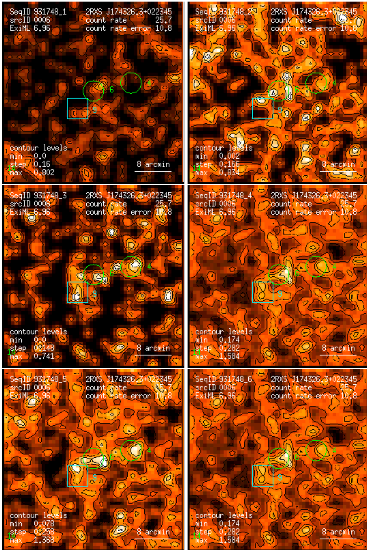
Figure 6: RASS 931748: detection 0006: band rate images, Gaussian filter: (1) PSPC channels 11 – 41, (2) 52 – 90, (3) 91 – 201, (4) 11 – 235, (5) 52 – 201, (6) 11 – 201. Broad band rates in counts/ks. Band rate contour levels in counts/ks/arcmin 2 .
