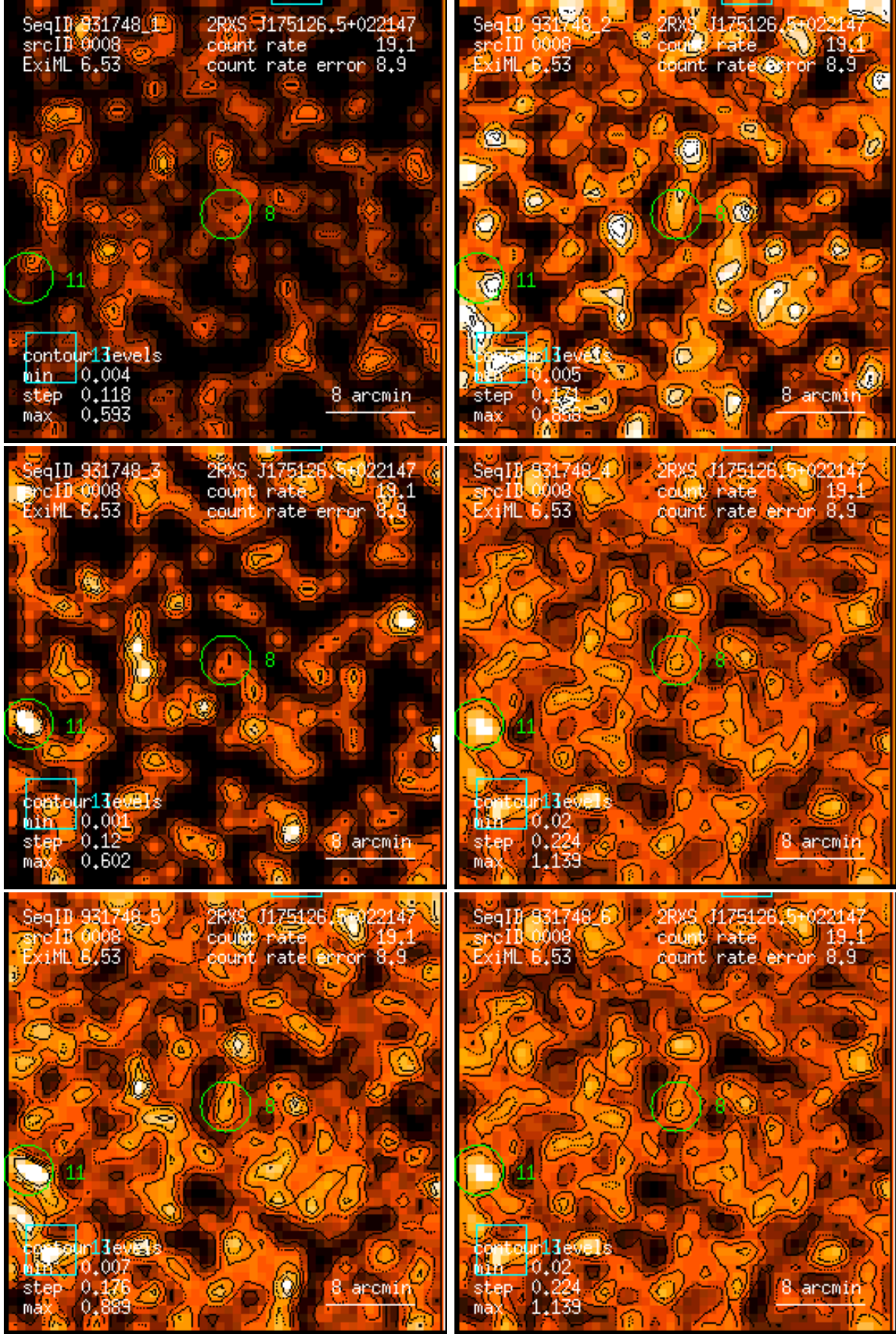
Figure 8: RASS 931748: detection 0008: band rate images, Gaussian filter: (1) PSPC channels 11 – 41, (2) 52 – 90, (3) 91 – 201, (4) 11 – 235, (5) 52 – 201, (6) 11 – 201. Broad band rates in counts/ks. Band rate contour levels in counts/ks/arcmin 2 .
