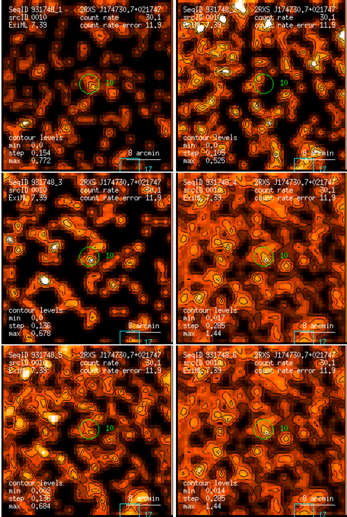
Figure 10: RASS 931748: detection 0010: band rate images, Gaussian filter: (1) PSPC channels 11 – 41, (2) 52 – 90, (3) 91 – 201, (4) 11 – 235, (5) 52 – 201, (6) 11 – 201. Broad band rates in counts/ks. Band rate contour levels in counts/ks/arcmin 2 .
