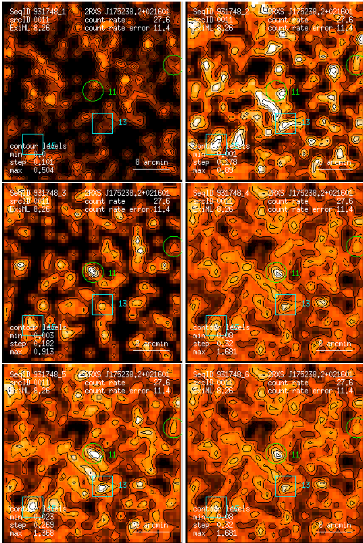
Figure 11: RASS 931748: detection 0011: band rate images, Gaussian filter: (1) PSPC channels 11 – 41, (2) 52 – 90, (3) 91 – 201, (4) 11 – 235, (5) 52 – 201, (6) 11 – 201. Broad band rates in counts/ks. Band rate contour levels in counts/ks/arcmin 2 .
