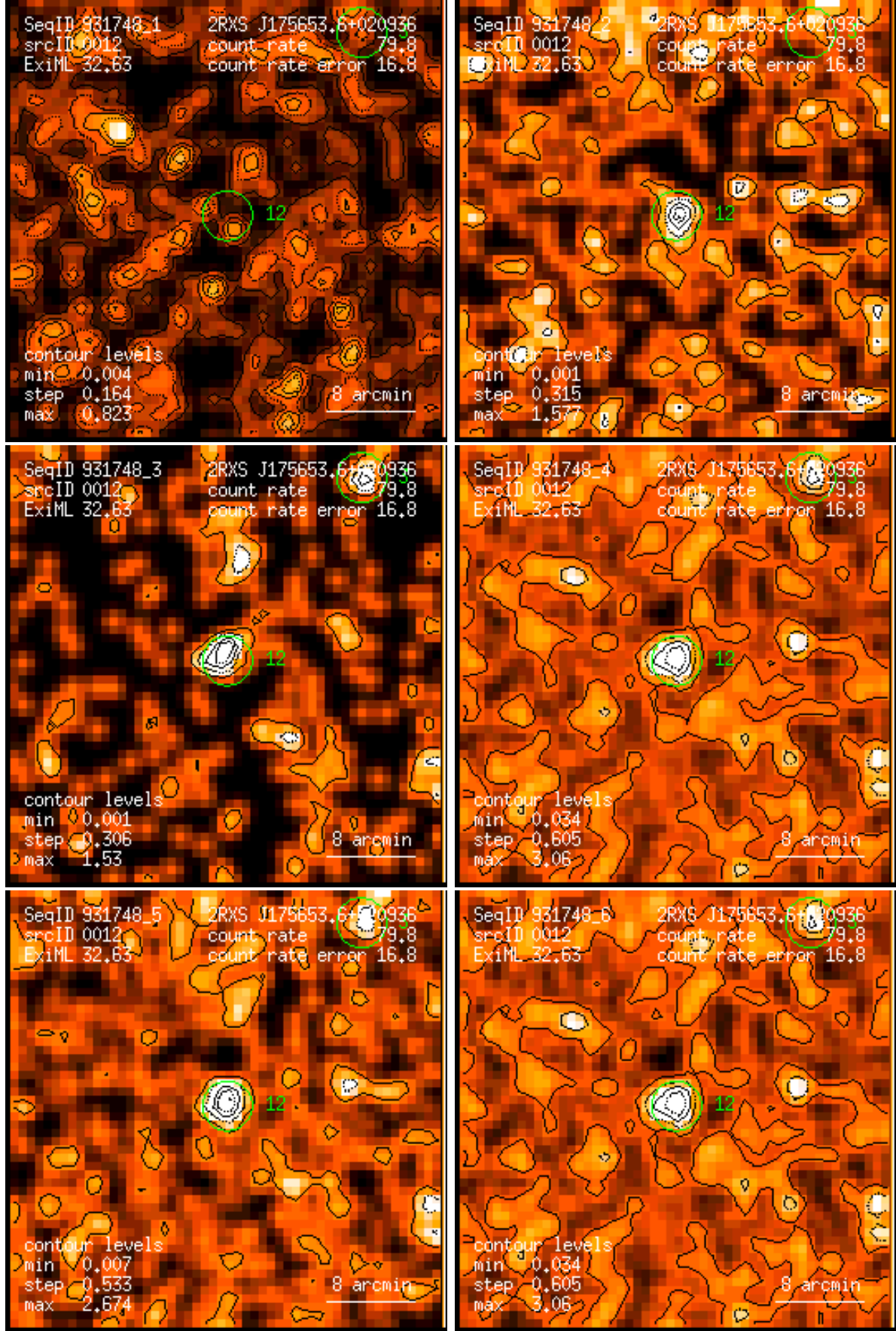
Figure 12: RASS 931748: detection 0012: band rate images, Gaussian filter: (1) PSPC channels 11 – 41, (2) 52 – 90, (3) 91 – 201, (4) 11 – 235, (5) 52 – 201, (6) 11 – 201. Broad band rates in counts/ks. Band rate contour levels in counts/ks/arcmin 2 .
