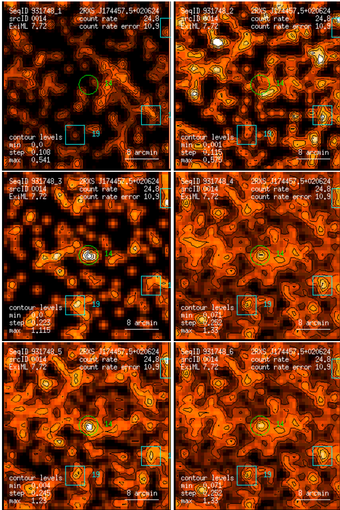
Figure 14: RASS 931748: detection 0014: band rate images, Gaussian filter: (1) PSPC channels 11 – 41, (2) 52 – 90, (3) 91 – 201, (4) 11 – 235, (5) 52 – 201, (6) 11 – 201. Broad band rates in counts/ks. Band rate contour levels in counts/ks/arcmin 2 .
