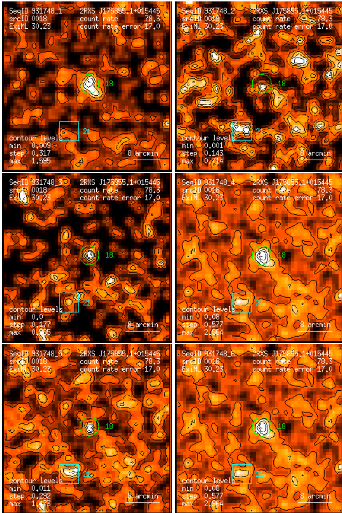
Figure 18: RASS 931748: detection 0018: band rate images, Gaussian filter: (1) PSPC channels 11 – 41, (2) 52 – 90, (3) 91 – 201, (4) 11 – 235, (5) 52 – 201, (6) 11 – 201. Broad band rates in counts/ks. Band rate contour levels in counts/ks/arcmin 2 .
