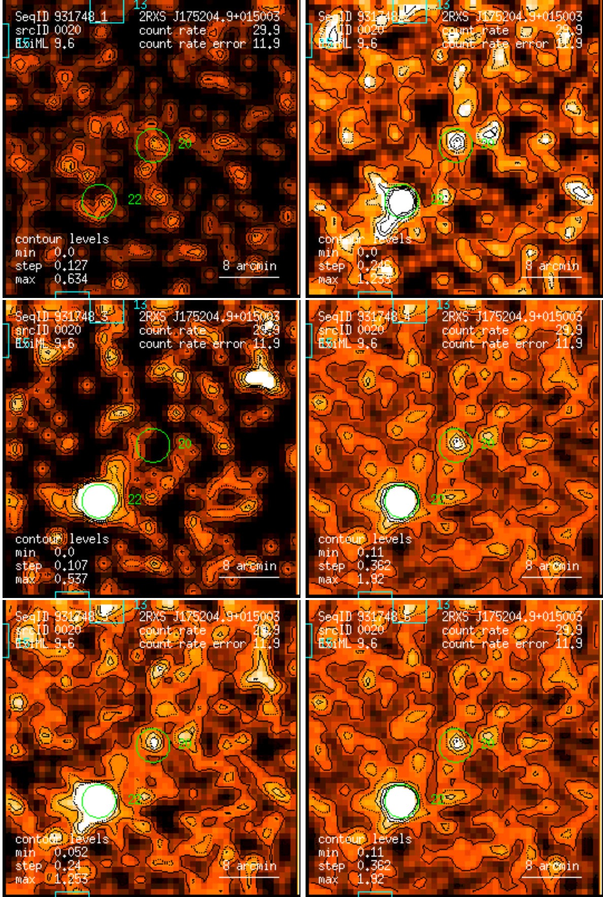
Figure 20: RASS 931748: detection 0020: band rate images, Gaussian filter: (1) PSPC channels 11 – 41, (2) 52 – 90, (3) 91 – 201, (4) 11 – 235, (5) 52 – 201, (6) 11 – 201. Broad band rates in counts/ks. Band rate contour levels in counts/ks/arcmin 2 .
