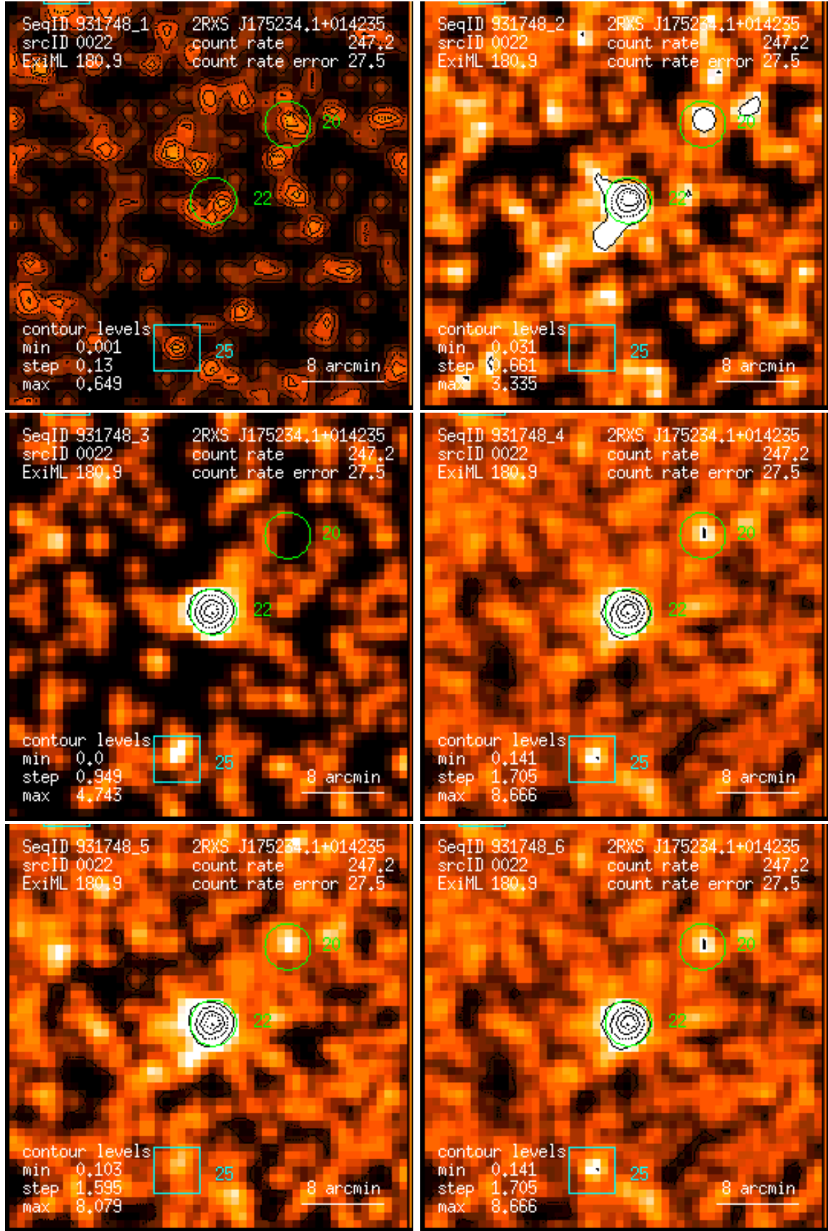
Figure 22: RASS 931748: detection 0022: band rate images, Gaussian filter: (1) PSPC channels 11 – 41, (2) 52 – 90, (3) 91 – 201, (4) 11 – 235, (5) 52 – 201, (6) 11 – 201. Broad band rates in counts/ks. Band rate contour levels in counts/ks/arcmin 2 .
