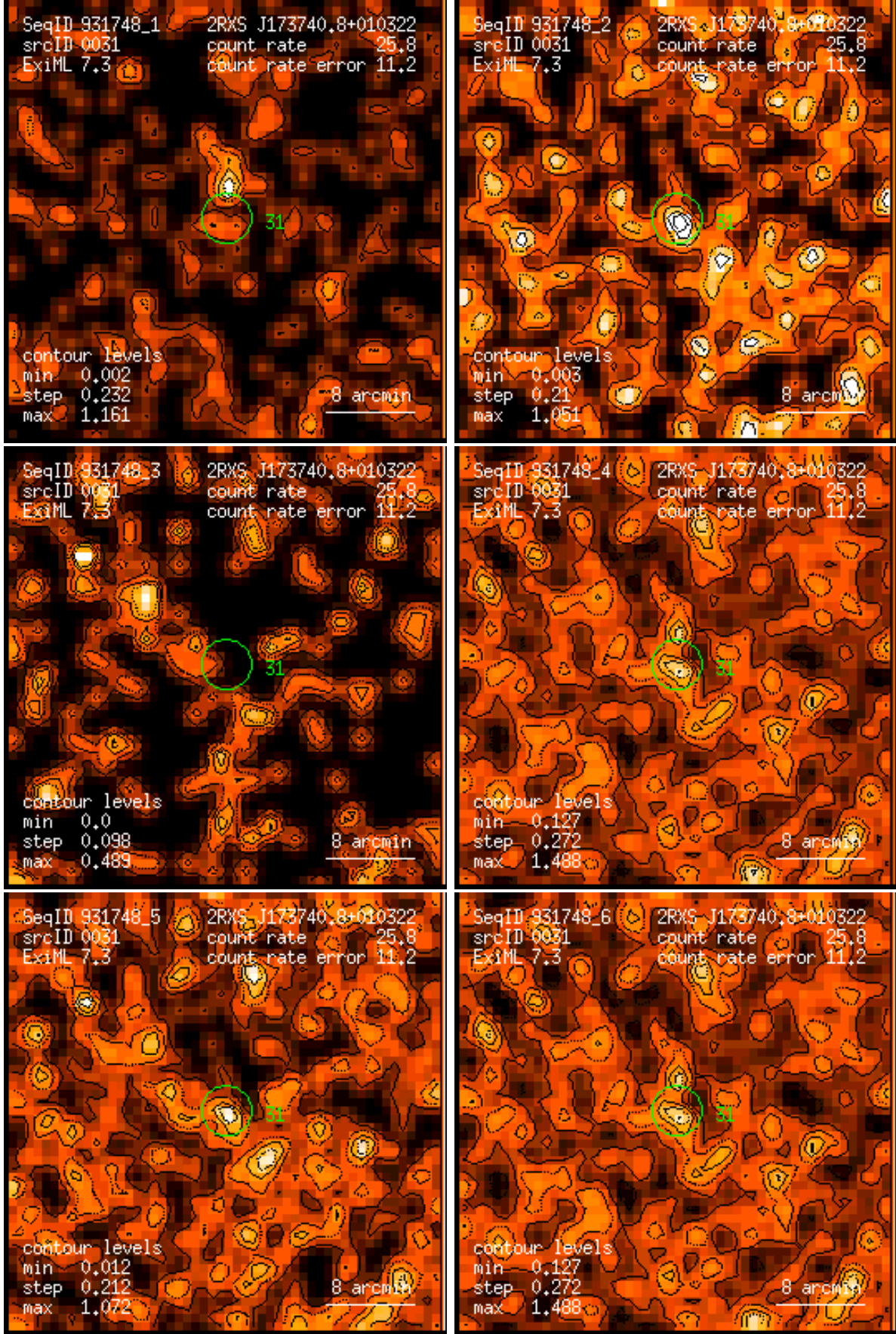
Figure 31: RASS 931748: detection 0031: band rate images, Gaussian filter: (1) PSPC channels 11 – 41, (2) 52 – 90, (3) 91 – 201, (4) 11 – 235, (5) 52 – 201, (6) 11 – 201. Broad band rates in counts/ks. Band rate contour levels in counts/ks/arcmin 2 .
