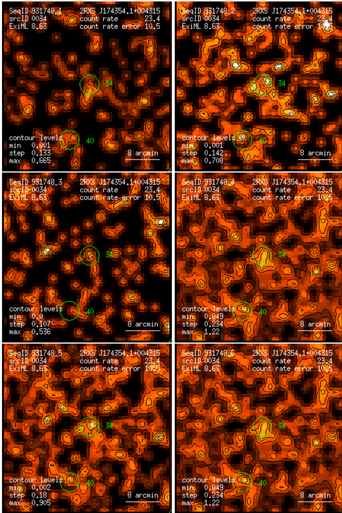
Figure 34: RASS 931748: detection 0034: band rate images, Gaussian filter: (1) PSPC channels 11 – 41, (2) 52 – 90, (3) 91 – 201, (4) 11 – 235, (5) 52 – 201, (6) 11 – 201. Broad band rates in counts/ks. Band rate contour levels in counts/ks/arcmin 2 .
