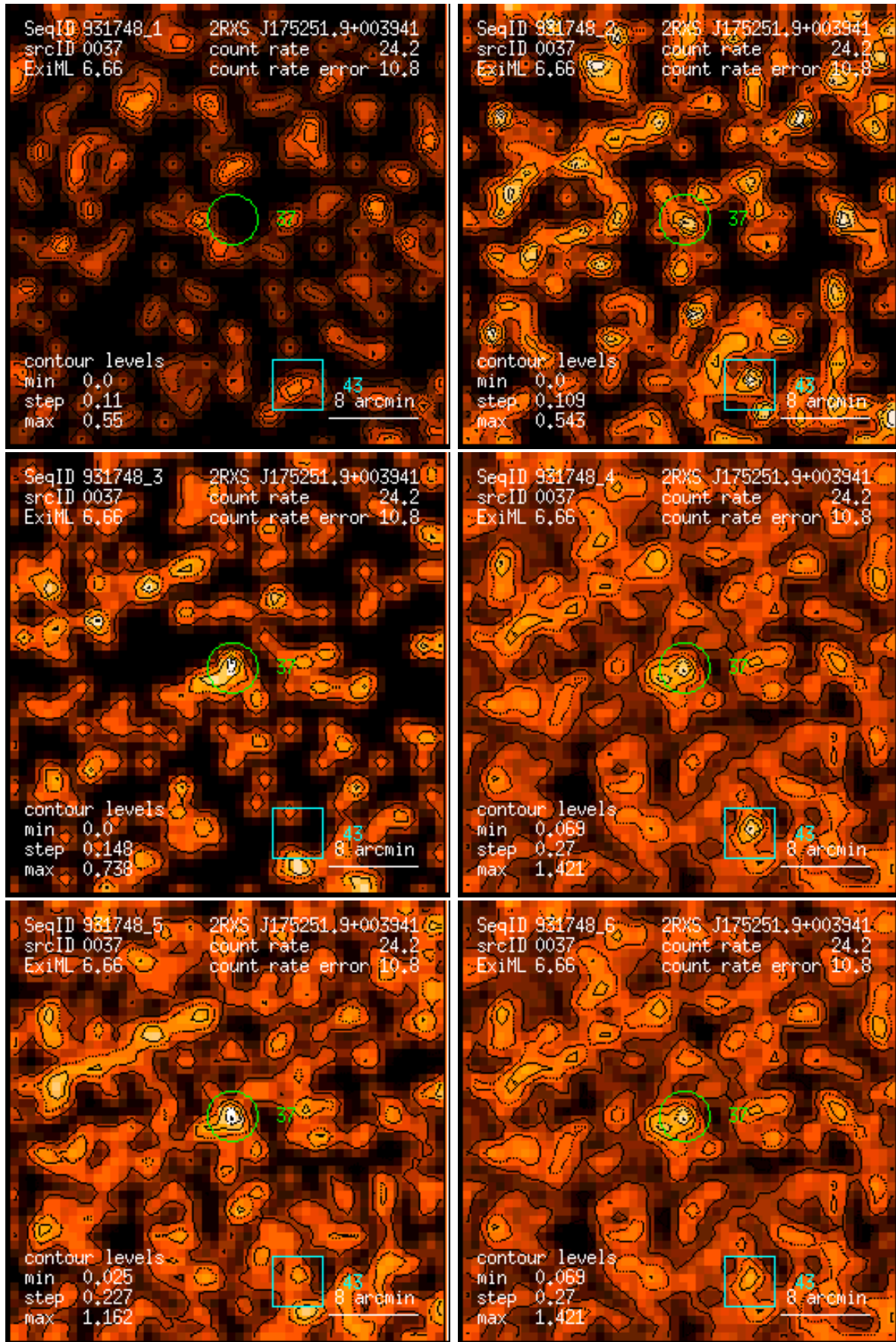
Figure 37: RASS 931748: detection 0037: band rate images, Gaussian filter: (1) PSPC channels 11 – 41, (2) 52 – 90, (3) 91 – 201, (4) 11 – 235, (5) 52 – 201, (6) 11 – 201. Broad band rates in counts/ks. Band rate contour levels in counts/ks/arcmin 2 .
