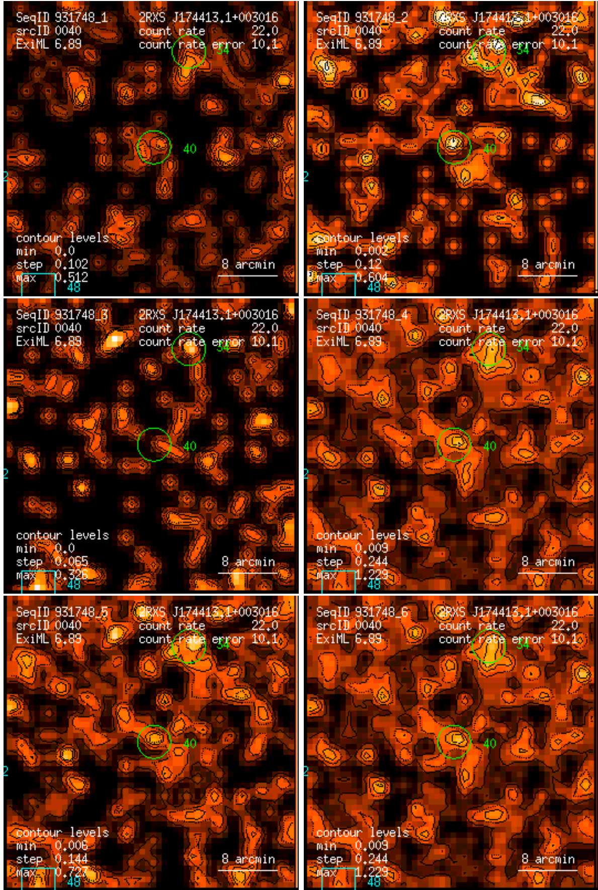
Figure 40: RASS 931748: detection 0040: band rate images, Gaussian filter: (1) PSPC channels 11 – 41, (2) 52 – 90, (3) 91 – 201, (4) 11 – 235, (5) 52 – 201, (6) 11 – 201. Broad band rates in counts/ks. Band rate contour levels in counts/ks/arcmin 2 .
