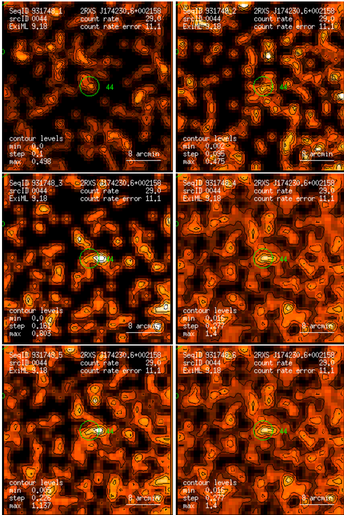
Figure 44: RASS 931748: detection 0044: band rate images, Gaussian filter: (1) PSPC channels 11 – 41, (2) 52 – 90, (3) 91 – 201, (4) 11 – 235, (5) 52 – 201, (6) 11 – 201. Broad band rates in counts/ks. Band rate contour levels in counts/ks/arcmin 2 .
