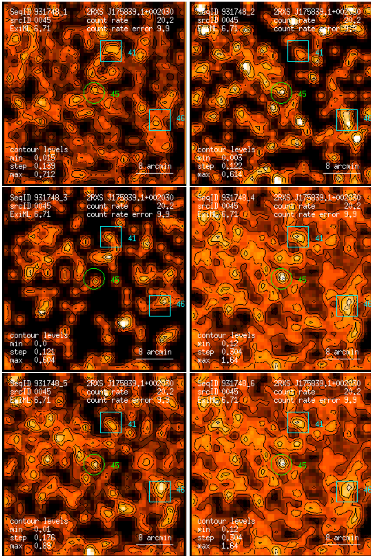
Figure 45: RASS 931748: detection 0045: band rate images, Gaussian filter: (1) PSPC channels 11 – 41, (2) 52 – 90, (3) 91 – 201, (4) 11 – 235, (5) 52 – 201, (6) 11 – 201. Broad band rates in counts/ks. Band rate contour levels in counts/ks/arcmin 2 .
