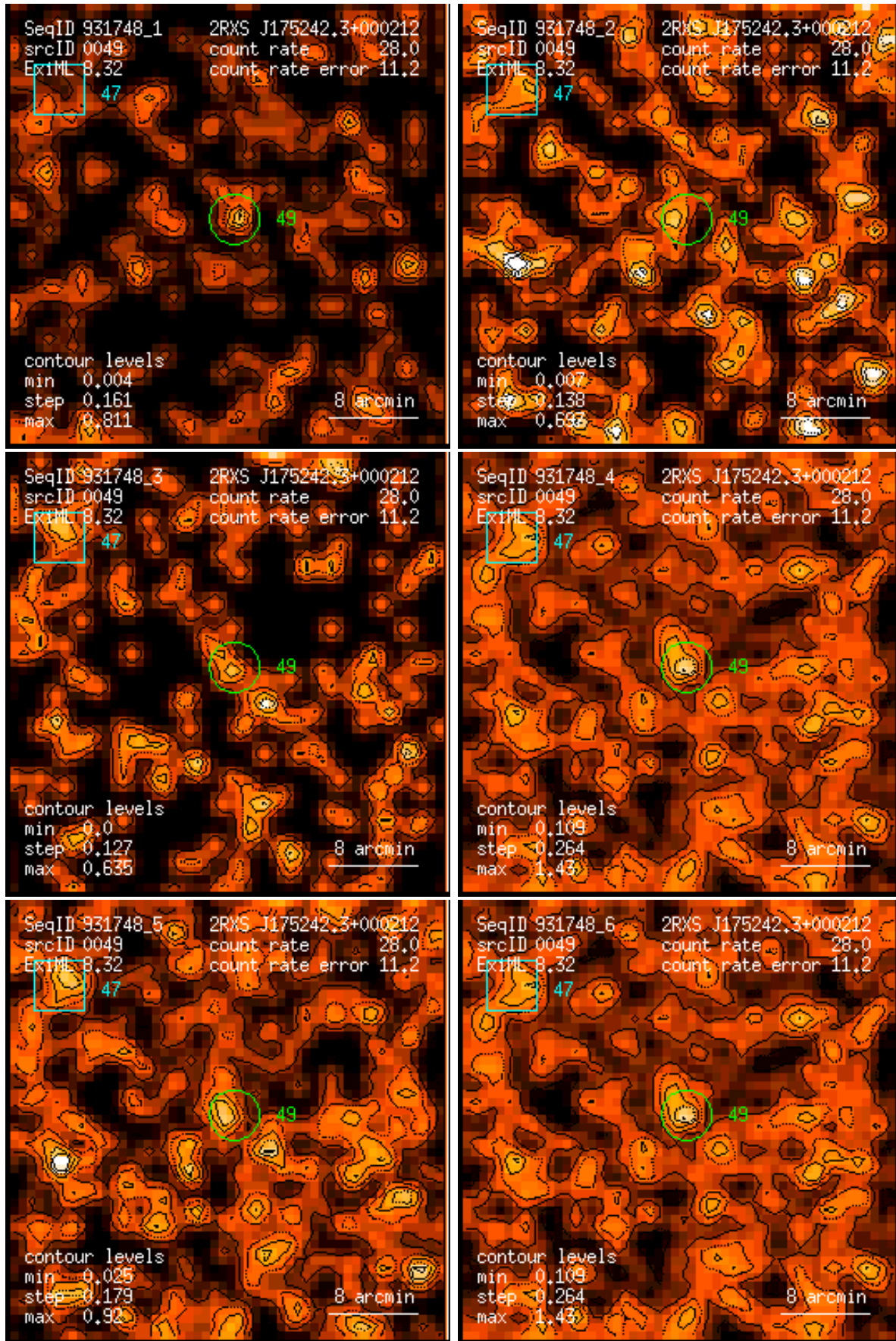
Figure 49: RASS 931748: detection 0049: band rate images, Gaussian filter: (1) PSPC channels 11 – 41, (2) 52 – 90, (3) 91 – 201, (4) 11 – 235, (5) 52 – 201, (6) 11 – 201. Broad band rates in counts/ks. Band rate contour levels in counts/ks/arcmin 2 .
