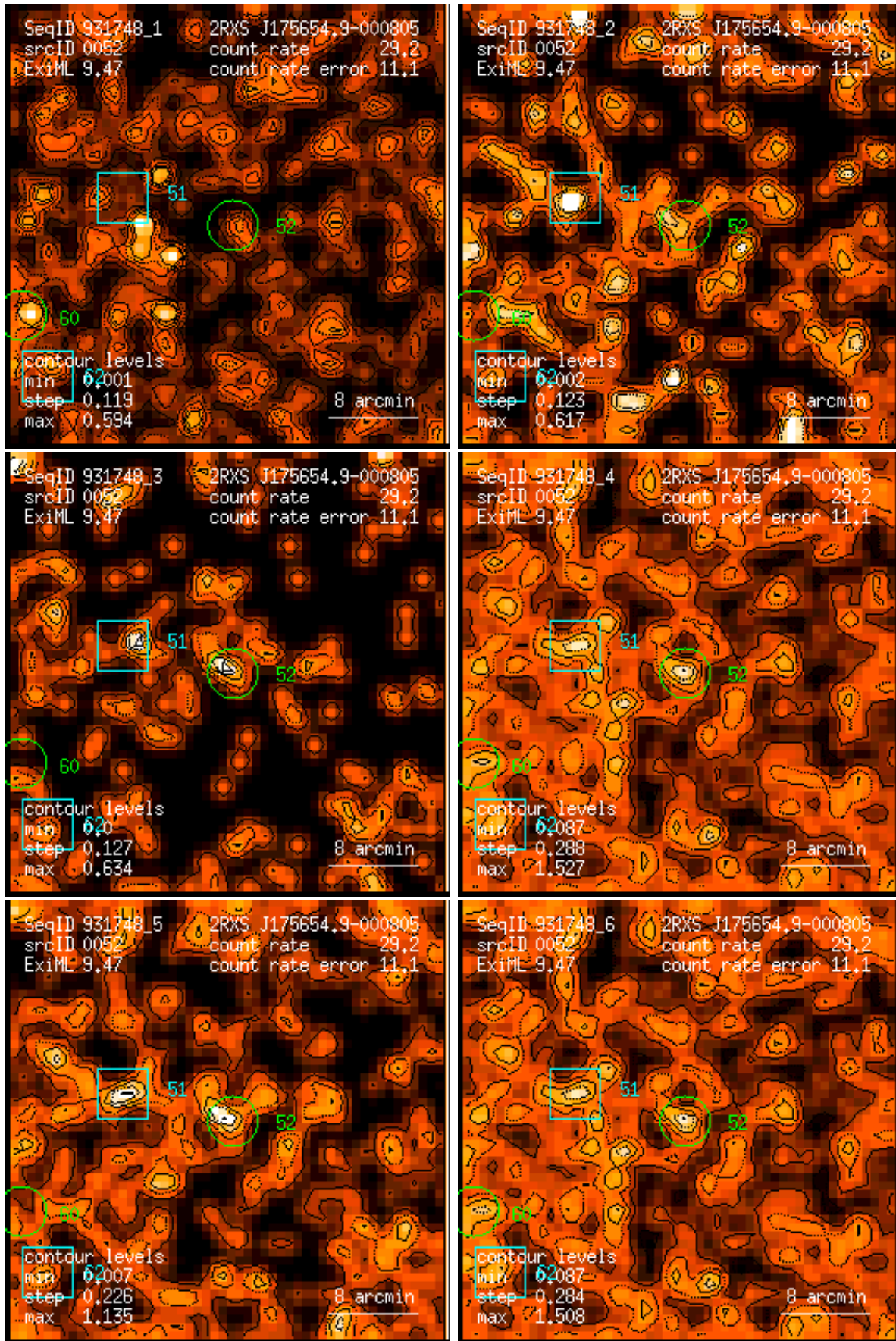
Figure 52: RASS 931748: detection 0052: band rate images, Gaussian filter: (1) PSPC channels 11 – 41, (2) 52 – 90, (3) 91 – 201, (4) 11 – 235, (5) 52 – 201, (6) 11 – 201. Broad band rates in counts/ks. Band rate contour levels in counts/ks/arcmin 2 .
