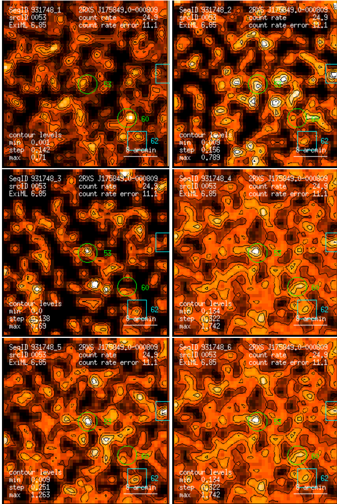
Figure 53: RASS 931748: detection 0053: band rate images, Gaussian filter: (1) PSPC channels 11 – 41, (2) 52 – 90, (3) 91 – 201, (4) 11 – 235, (5) 52 – 201, (6) 11 – 201. Broad band rates in counts/ks. Band rate contour levels in counts/ks/arcmin 2 .
