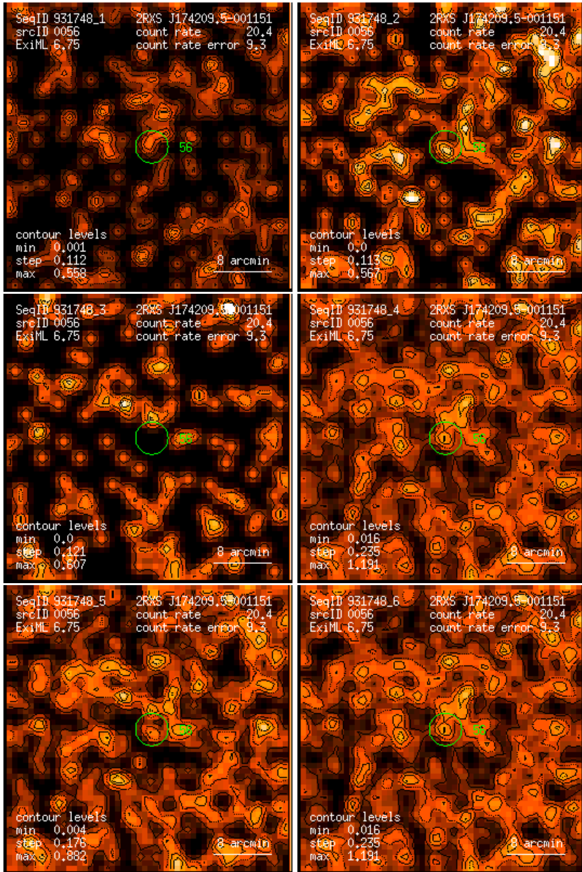
Figure 56: RASS 931748: detection 0056: band rate images, Gaussian filter: (1) PSPC channels 11 – 41, (2) 52 – 90, (3) 91 – 201, (4) 11 – 235, (5) 52 – 201, (6) 11 – 201. Broad band rates in counts/ks. Band rate contour levels in counts/ks/arcmin 2 .
