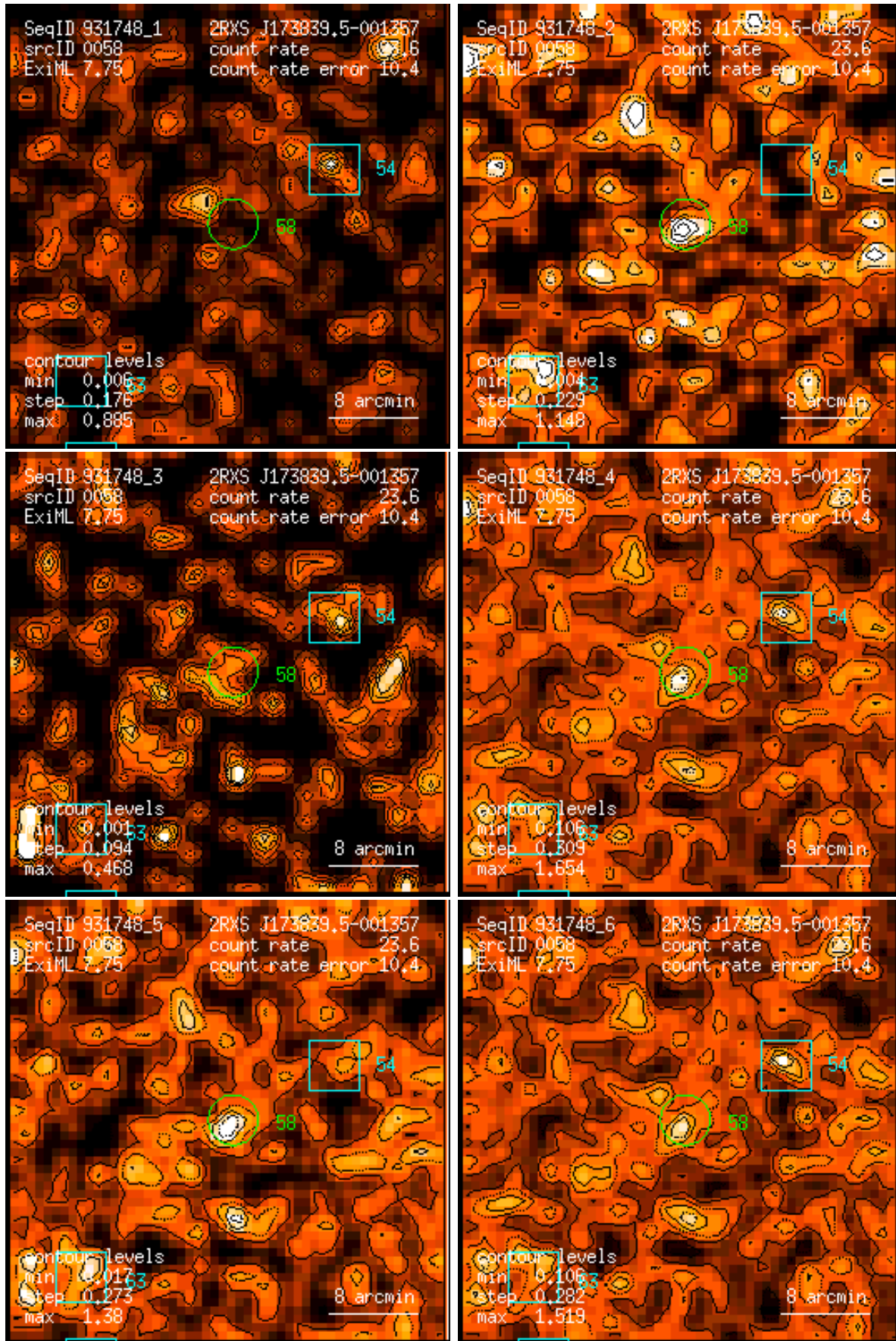
Figure 58: RASS 931748: detection 0058: band rate images, Gaussian filter: (1) PSPC channels 11 – 41, (2) 52 – 90, (3) 91 – 201, (4) 11 – 235, (5) 52 – 201, (6) 11 – 201. Broad band rates in counts/ks. Band rate contour levels in counts/ks/arcmin 2 .
