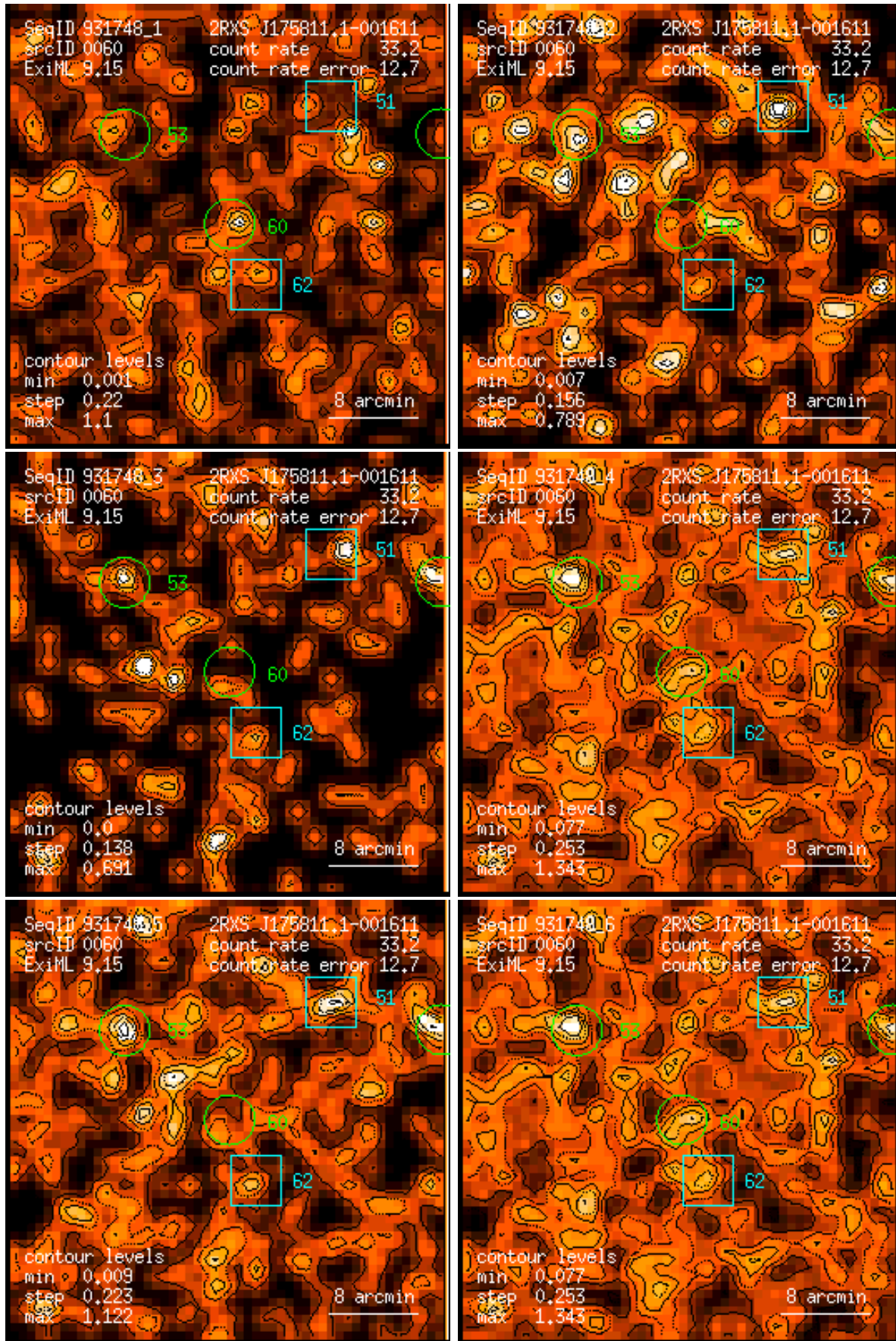
Figure 60: RASS 931748: detection 0060: band rate images, Gaussian filter: (1) PSPC channels 11 – 41, (2) 52 – 90, (3) 91 – 201, (4) 11 – 235, (5) 52 – 201, (6) 11 – 201. Broad band rates in counts/ks. Band rate contour levels in counts/ks/arcmin 2 .
