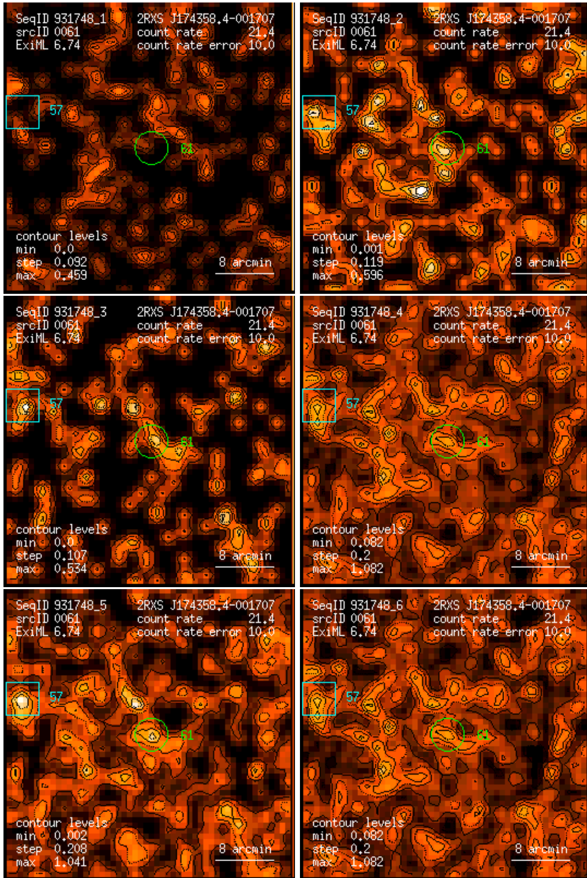
Figure 61: RASS 931748: detection 0061: band rate images, Gaussian filter: (1) PSPC channels 11 – 41, (2) 52 – 90, (3) 91 – 201, (4) 11 – 235, (5) 52 – 201, (6) 11 – 201. Broad band rates in counts/ks. Band rate contour levels in counts/ks/arcmin 2 .
