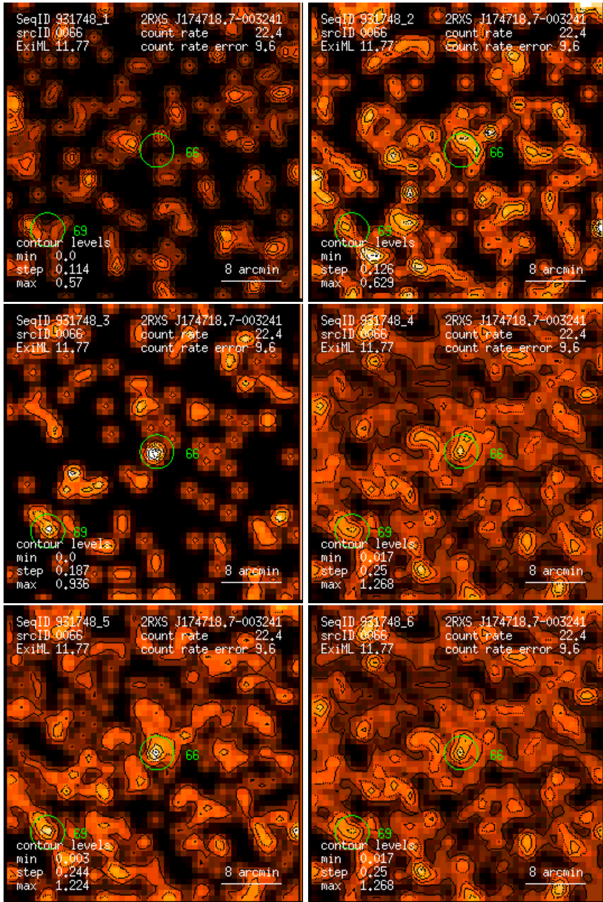
Figure 66: RASS 931748: detection 0066: band rate images, Gaussian filter: (1) PSPC channels 11 – 41, (2) 52 – 90, (3) 91 – 201, (4) 11 – 235, (5) 52 – 201, (6) 11 – 201. Broad band rates in counts/ks. Band rate contour levels in counts/ks/arcmin 2 .
