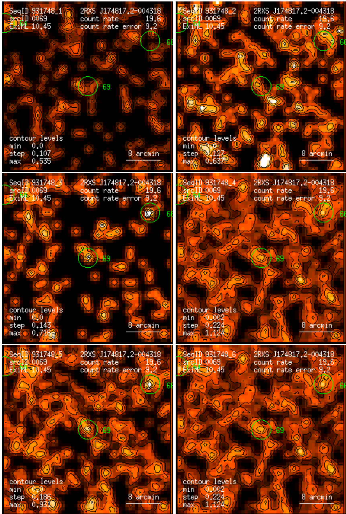
Figure 69: RASS 931748: detection 0069: band rate images, Gaussian filter: (1) PSPC channels 11 – 41, (2) 52 – 90, (3) 91 – 201, (4) 11 – 235, (5) 52 – 201, (6) 11 – 201. Broad band rates in counts/ks. Band rate contour levels in counts/ks/arcmin 2 .
