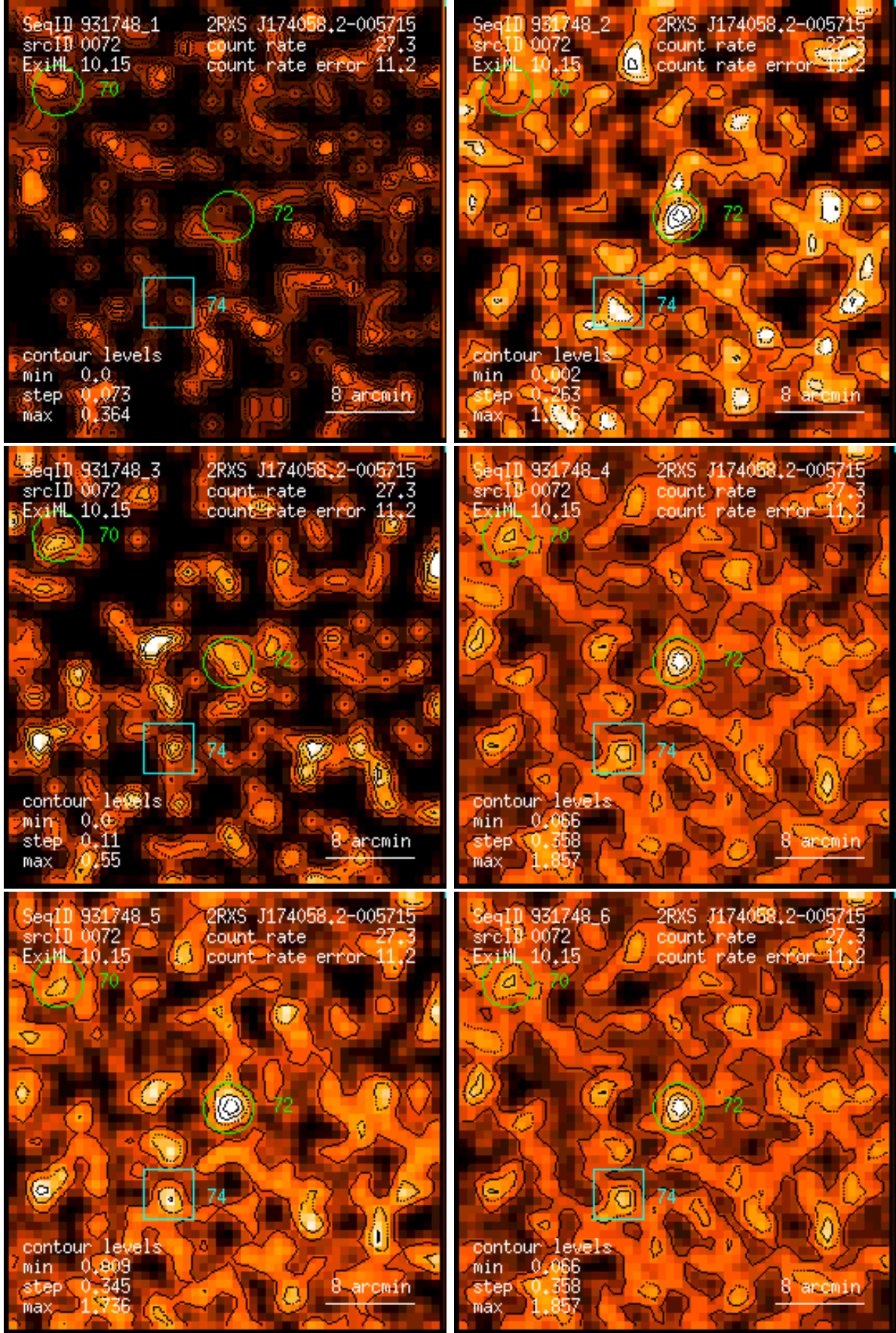
Figure 72: RASS 931748: detection 0072: band rate images, Gaussian filter: (1) PSPC channels 11 – 41, (2) 52 – 90, (3) 91 – 201, (4) 11 – 235, (5) 52 – 201, (6) 11 – 201. Broad band rates in counts/ks. Band rate contour levels in counts/ks/arcmin 2 .
