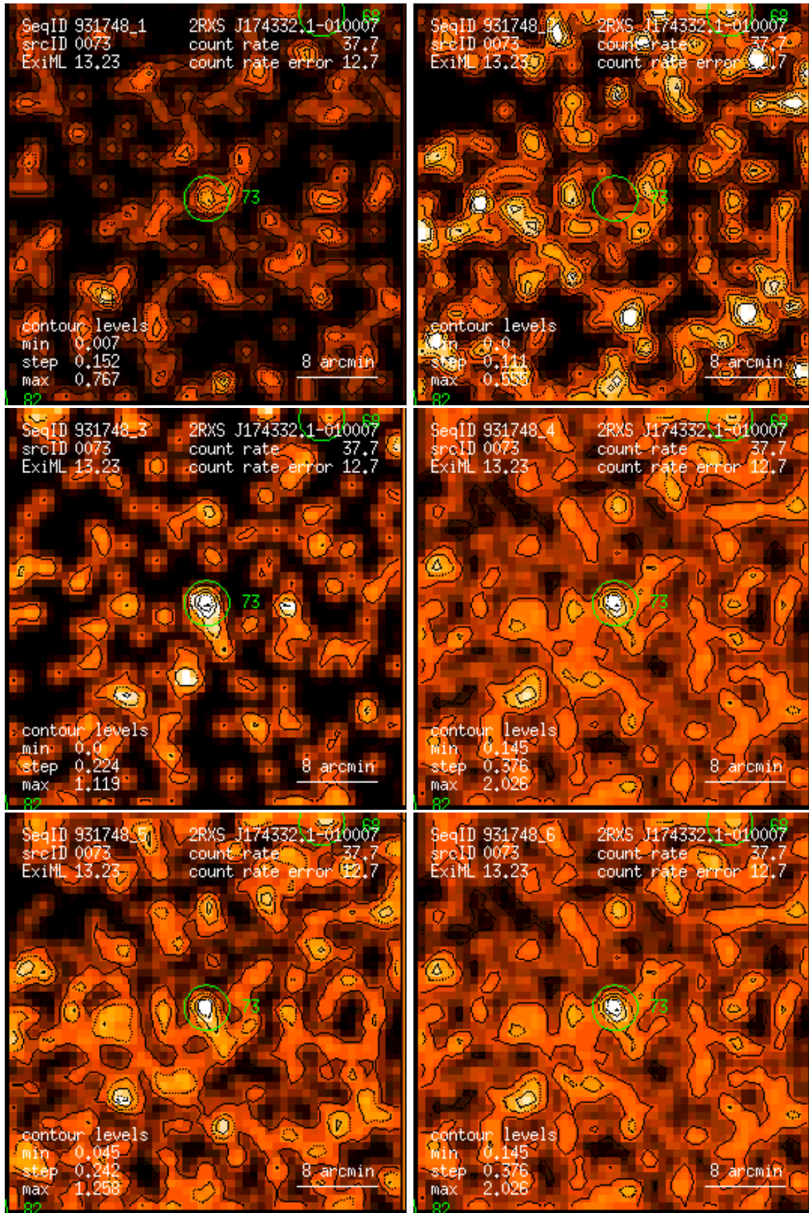
Figure 73: RASS 931748: detection 0073: band rate images, Gaussian filter: (1) PSPC channels 11 – 41, (2) 52 – 90, (3) 91 – 201, (4) 11 – 235, (5) 52 – 201, (6) 11 – 201. Broad band rates in counts/ks. Band rate contour levels in counts/ks/arcmin 2 .
